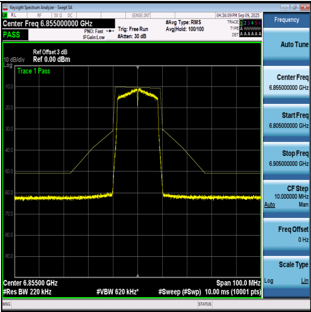
NTNV-11A-Ant1+2-6855-PASS
