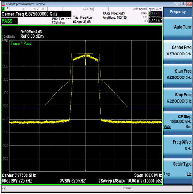
NTNV-11A-Ant1+2-6875-PASS
