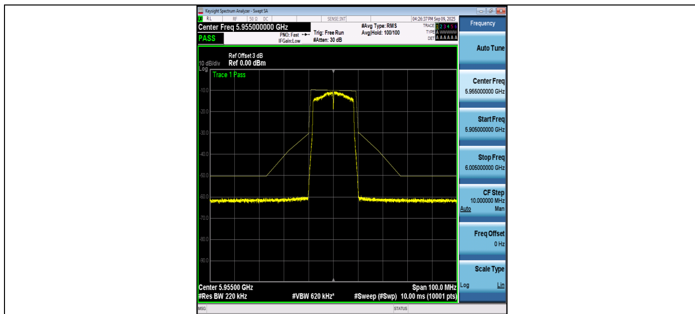
NTNV-11A-Ant1+2-5955-PASS
