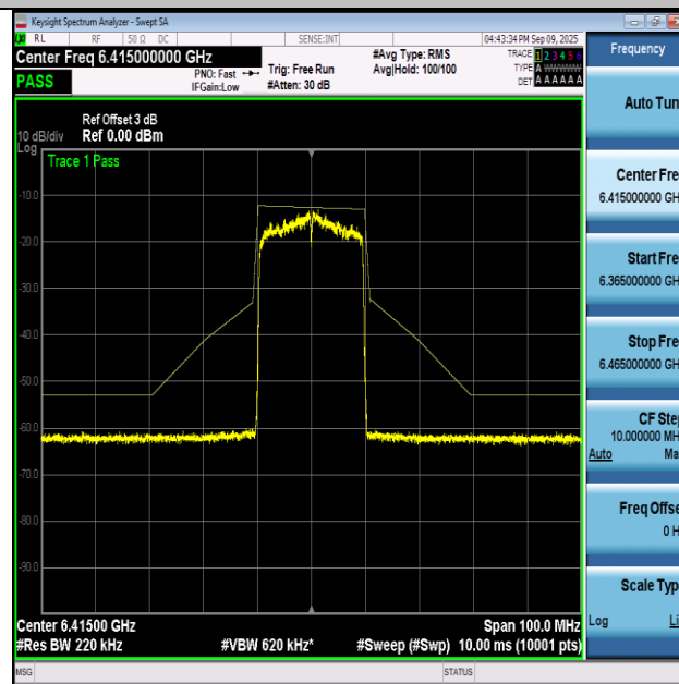
NTNV-11AX20-Ant1+2-6415-PASS
