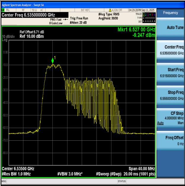
11AX20-Ant1+2-6535-52Tone-RU37-PASS
