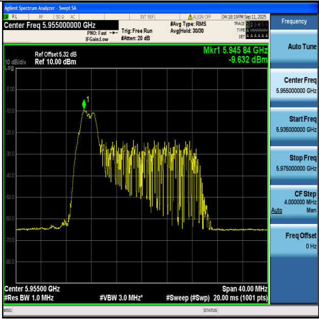
11AX20-Ant1+2-5955-26Tone-RU0-PASS
