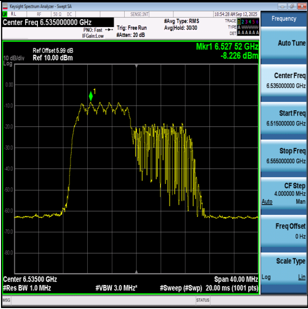
11AX20-Ant1+2-6535-106Tone-RU53-PASS
