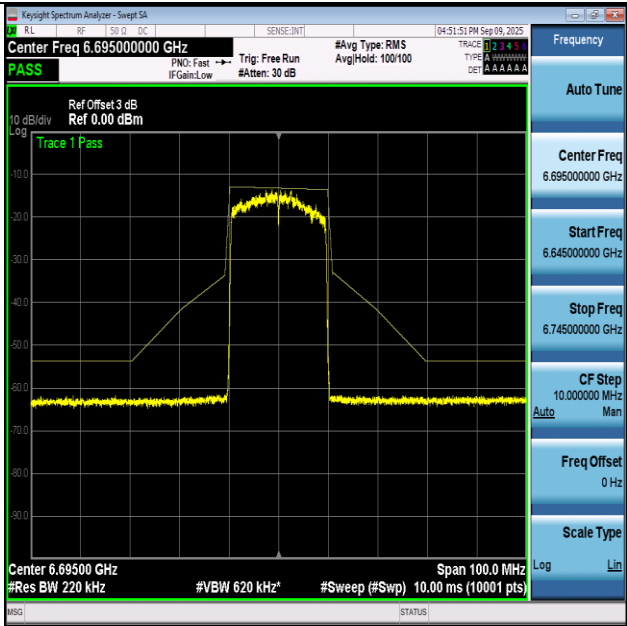
NITNV-11AX20-Ant1+2-6695-PASS
