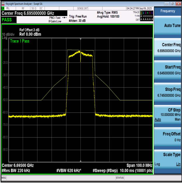
NTNV-11A-Ant1+2-6695-PASS
