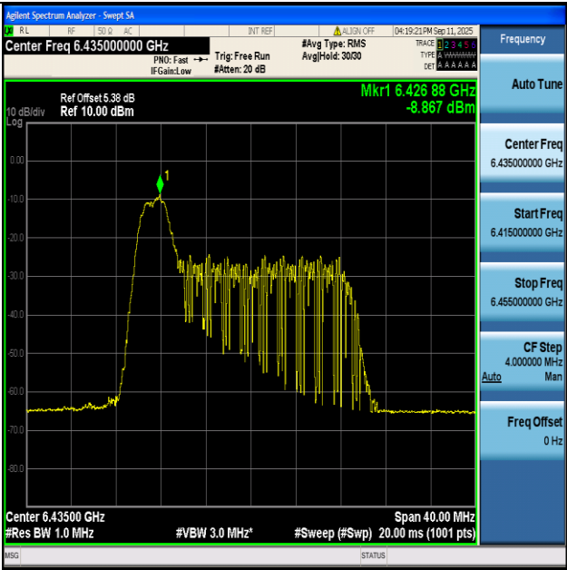
11AX20-Ant1+2-6435-26Tone-RU0-PASS
