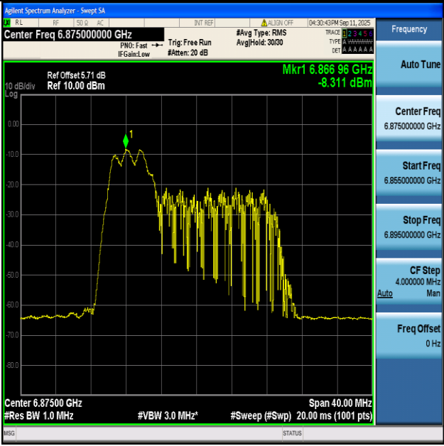
11AX20-Ant1+2-6875-52Tone-RU37-PASS
