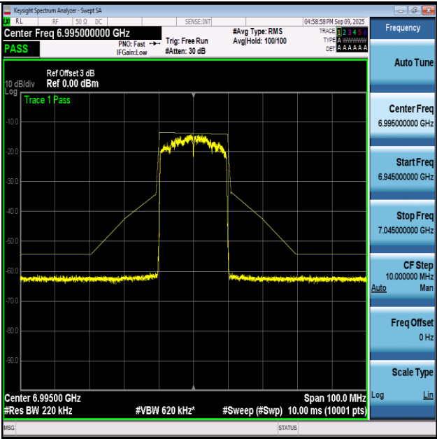
NTNV-11AX20-Ant1+2-6995-PASS
