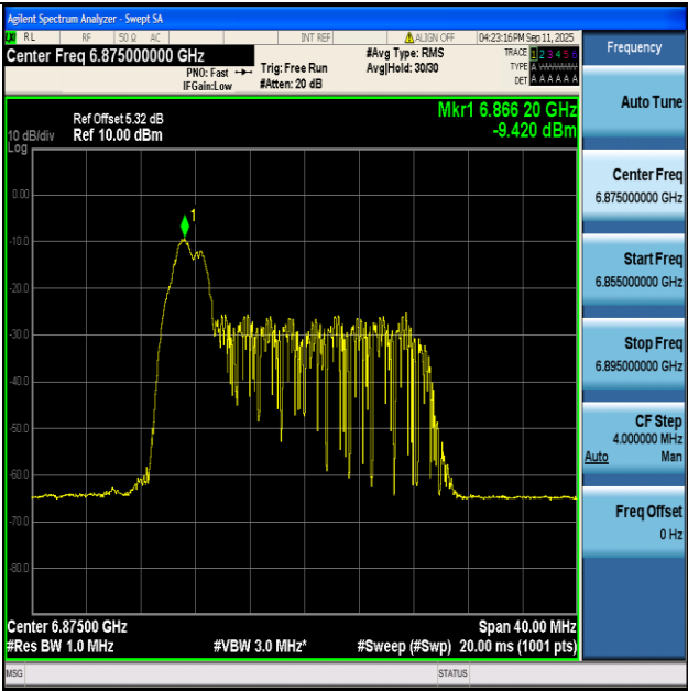
11AX20-Ant1+2-6875-26Tone-RU0-PASS
