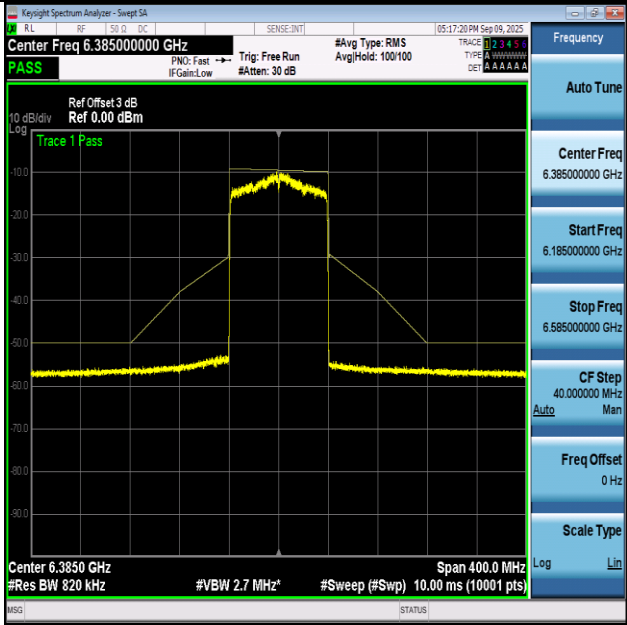
NITNV-11AX80-Ant1+2-6385-PASS
