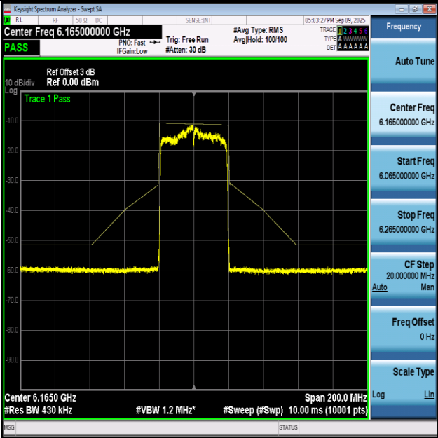
NTVN-11AX40-Ant1+2-6165-PASS
