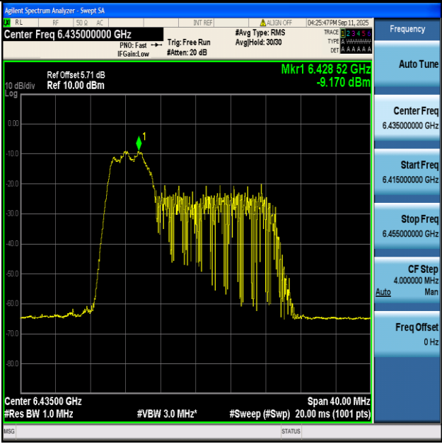
11AX20-Ant1+2-6435-52Tone-RU37-PASS
