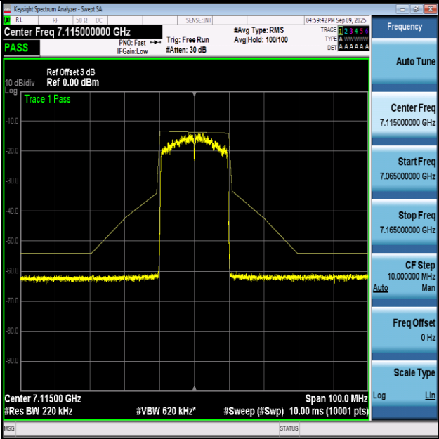
NTNV-11AX20-Ant1+2-7115-PASS
