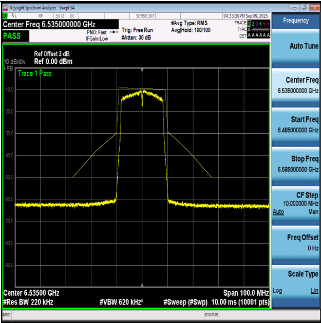
NTNV-11A-Ant1+2-6535-PASS
