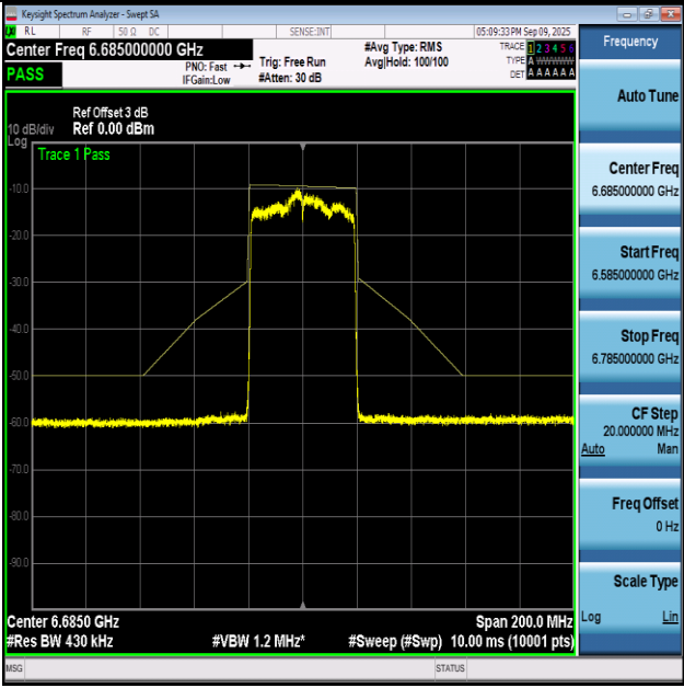
NTVN-11AX40-Ant1+2-6685-PASS
