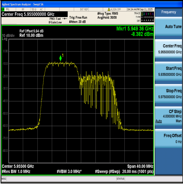
11AX20-Ant1+2-5955-106Tone-RU53-PASS
