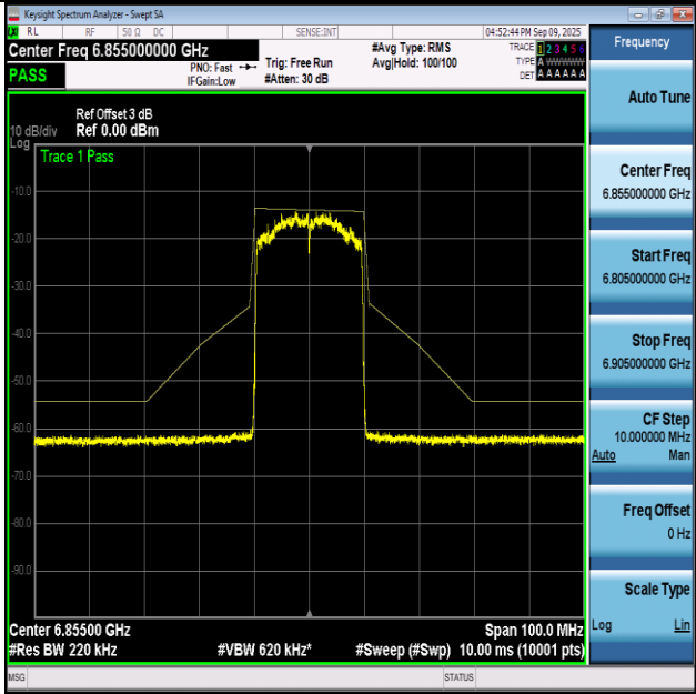
NITNV-11AX20-Ant1+2-6855-PASS
