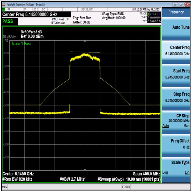
NITNV-11AX80-Ant1+2-6145-PASS
