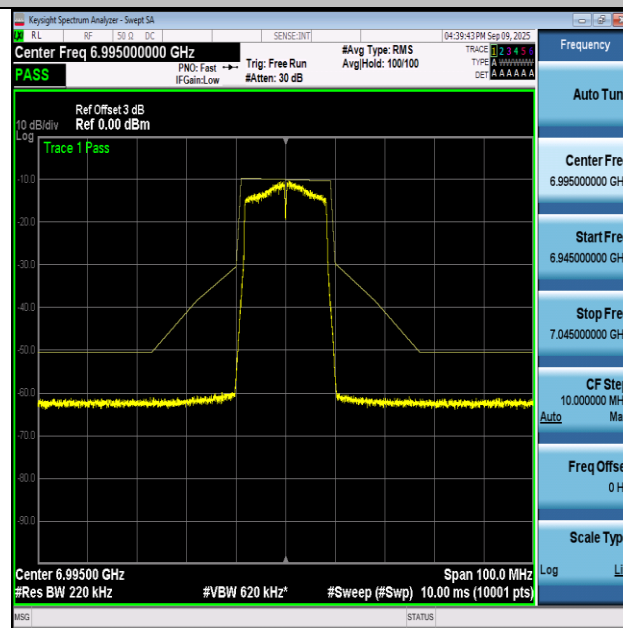
NTNV-11A-Ant1+2-6995-PASS
