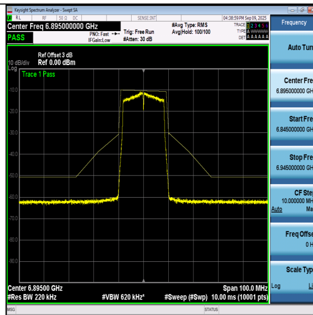
NTNV-11A-Ant1+2-6895-PASS
