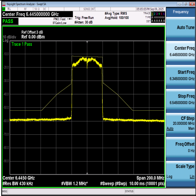
NTVN-11AX40-Ant1+2-6445-PASS
