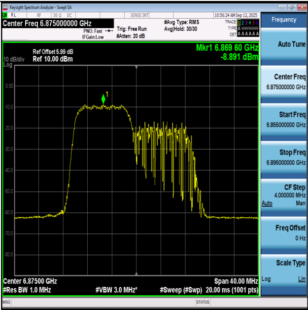
11AX20-Ant1+2-6875-106Tone-RU53-PASS
