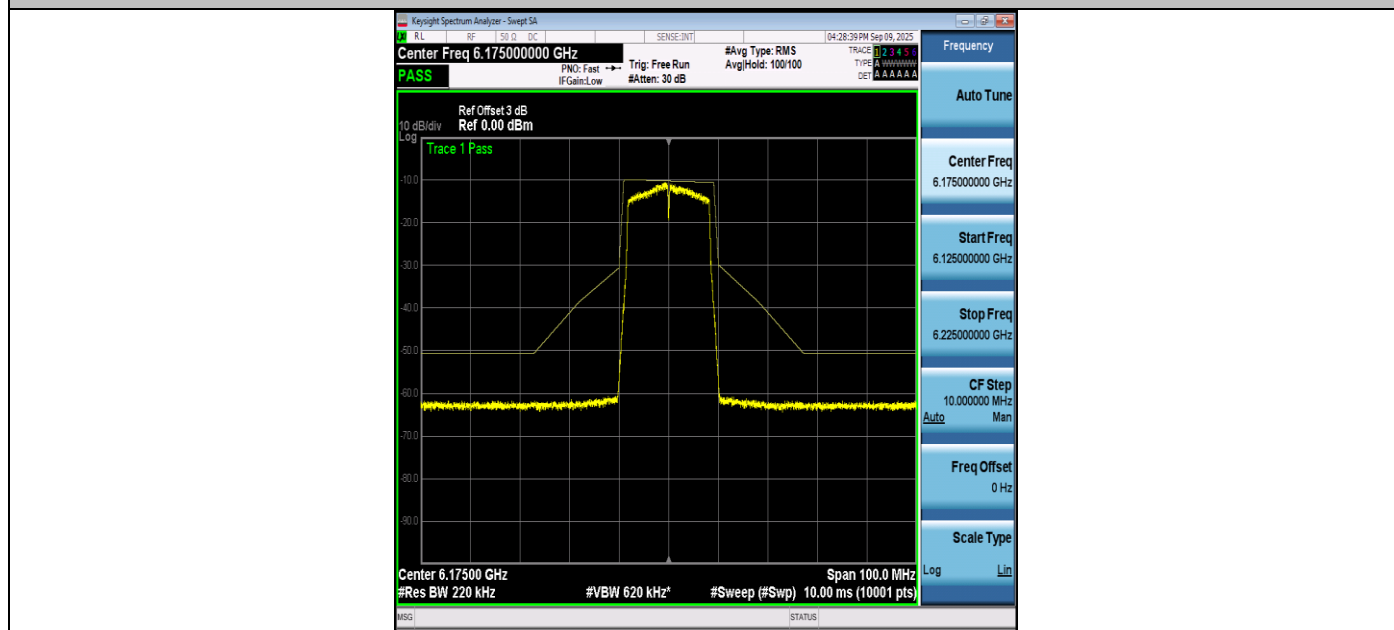
NTNV-11A-Ant1+2-6175-PASS
