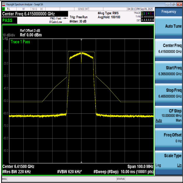
NTNV-11A-Ant1+2-6415-PASS
