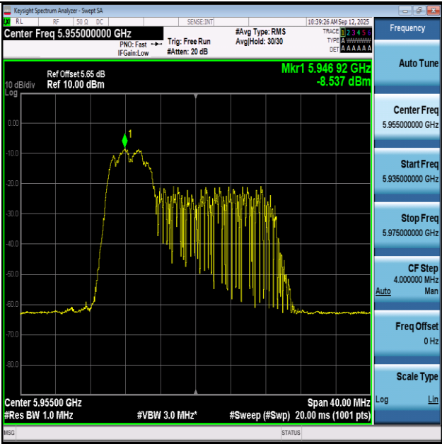
11AX20-Ant1+2-5955-52Tone-RU37-PASS
