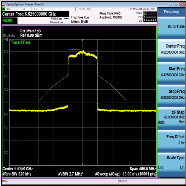
NTVN-11AX80-Ant1+2-6625-PASS
