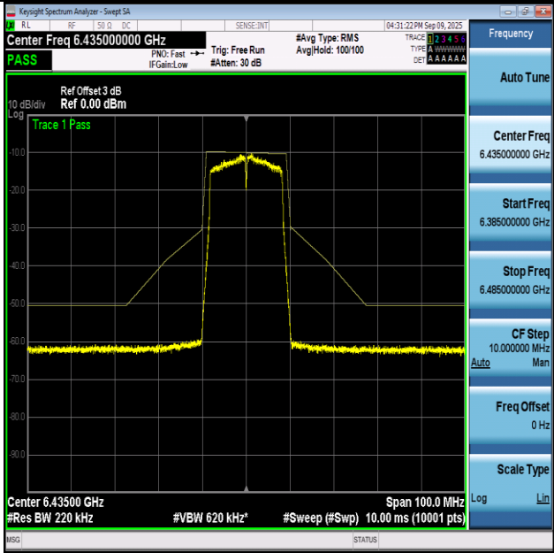
NTNV-11A-Ant1+2-6435-PASS
