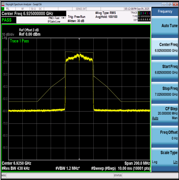
NTVN-11AX40-Ant1+2-6925-PASS
