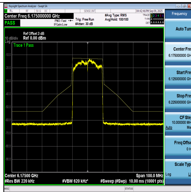
NTNV-11AX20-Ant1+2-6175-PASS
