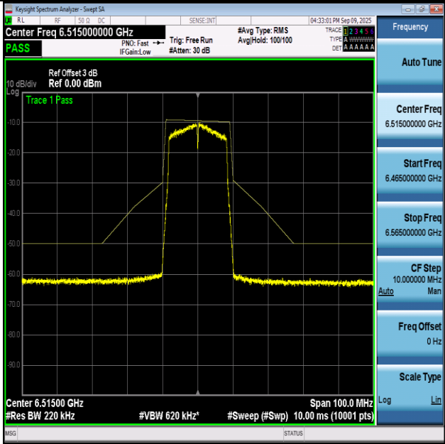
NTVN-11A-Ant1+2-6515-PASS
