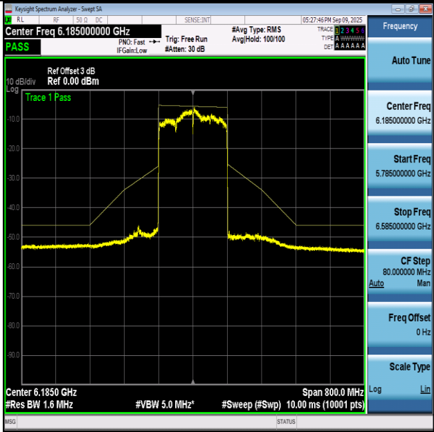
NTNV-11AX160-Ant1+2-6185-PASS
