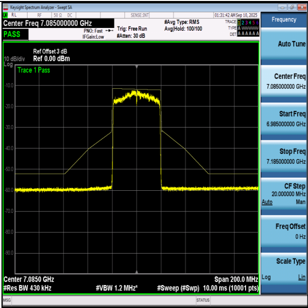
NTNV-11BE40-Ant1+2-7085-PASS
