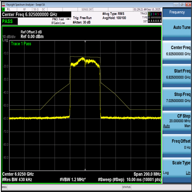
NTNV-11BE40-Ant1+2-6925-PASS
