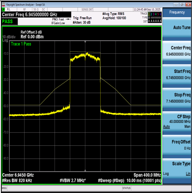
NTNV-11BE80-Ant1+2-6945-PASS
