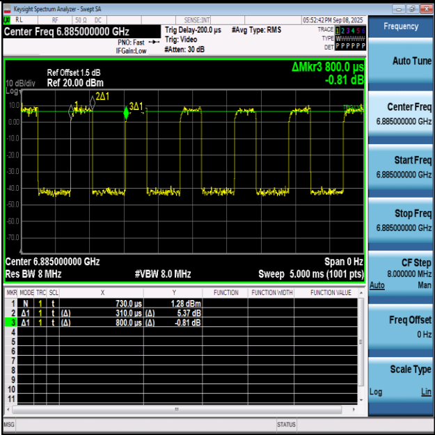
NTNV-11AX40SISO-Ant1-6885
