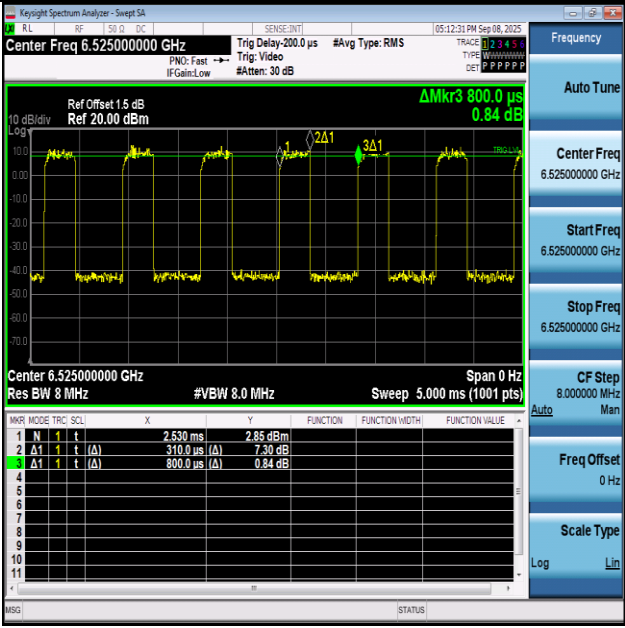
NTNV-11AX40SISO-Ant1-6525
