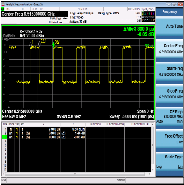
NTNV-11AX20SISO-Ant1-6515
