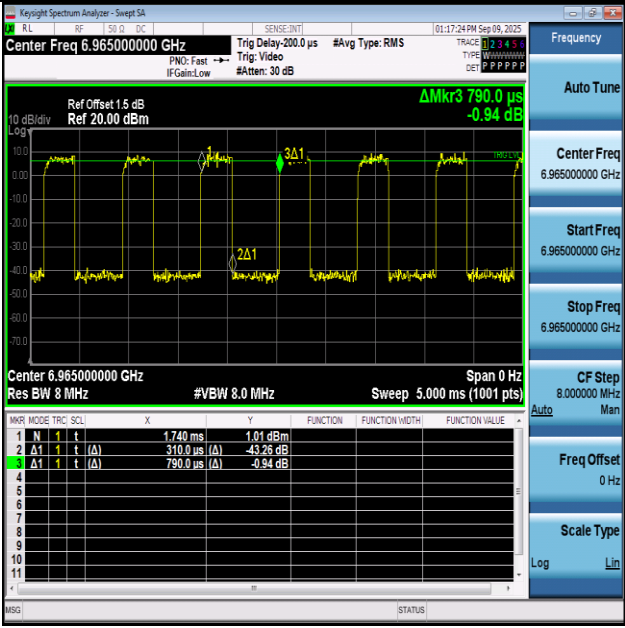
NTNV-11AX40SISO-Ant1-6965
