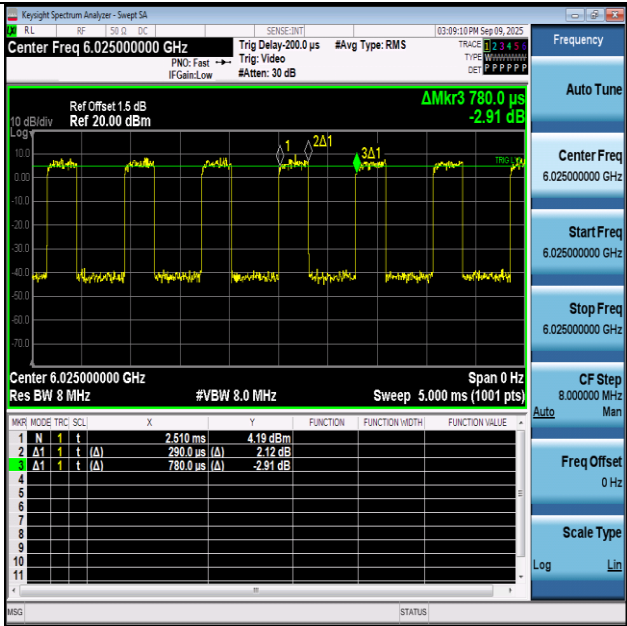
NTNV-11AX160SISO-Ant1-6025
