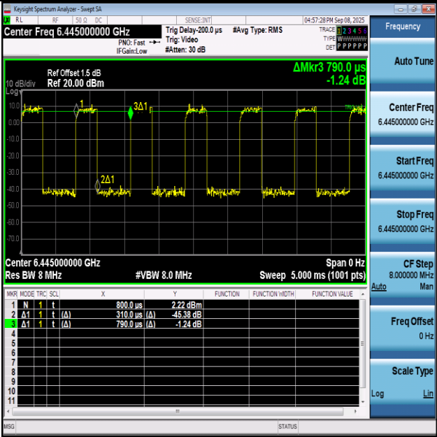
NTNV-11AX40SISO-Ant1-6445
