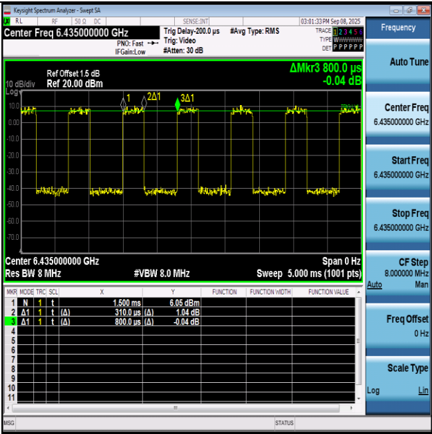
NTNV-11AX20SISO-Ant1-6435
