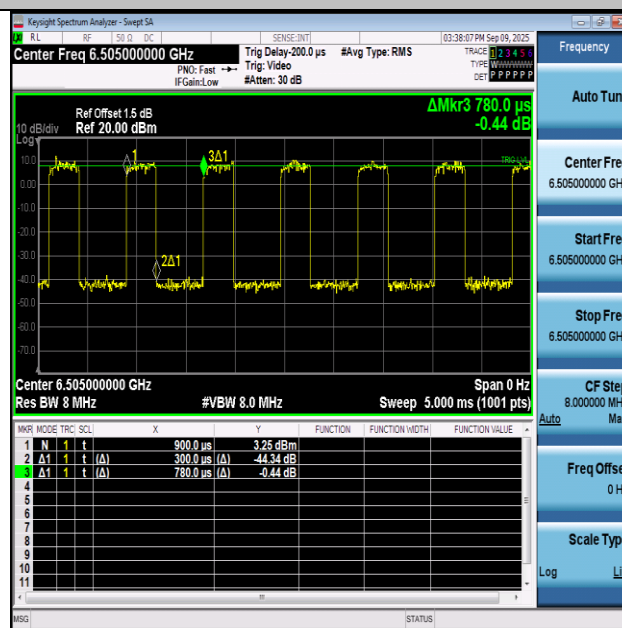
NTNV-11AX160SISO-Ant1-6505
