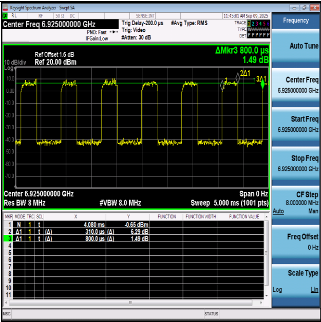
NTNV-11AX40SISO-Ant1-6925
