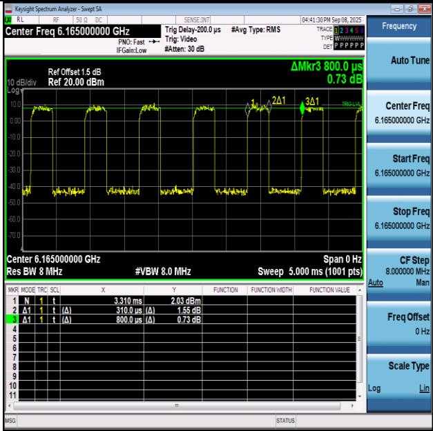
NTNV-11AX40SISO-Ant1-6165
