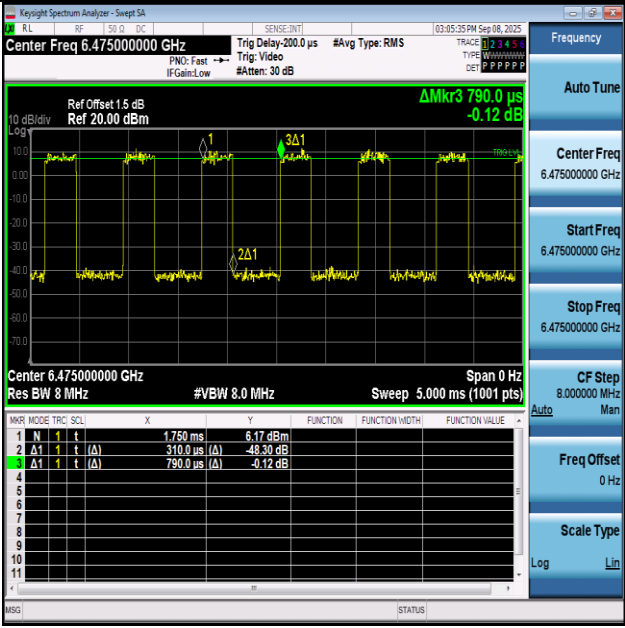
NTNV-11AX20SISO-Ant1-6475
