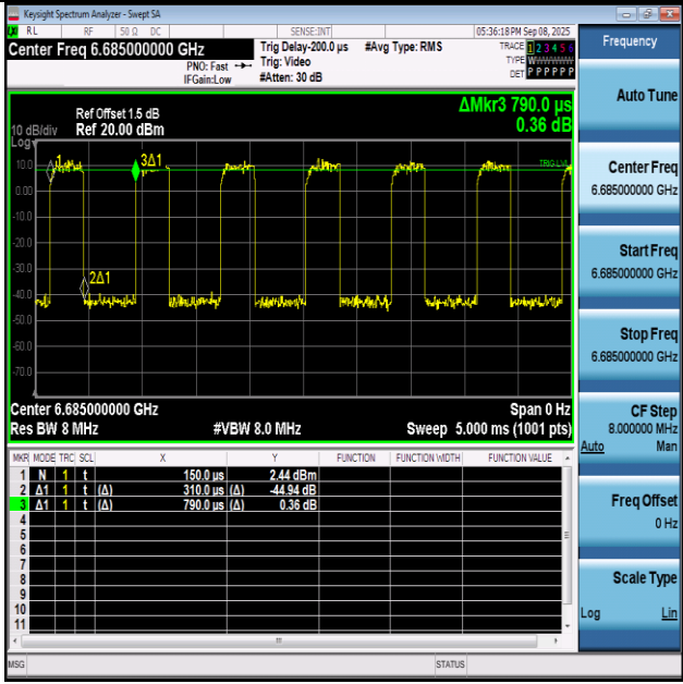
NTNV-11AX40SISO-Ant1-6685
