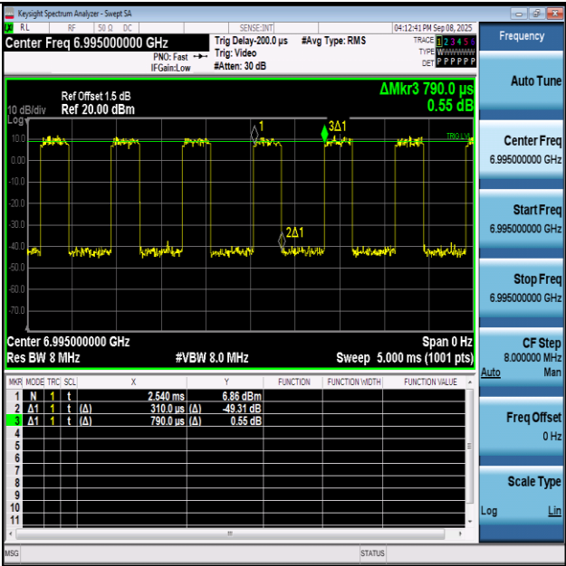
NTNV-11AX20SISO-Ant1-6995
