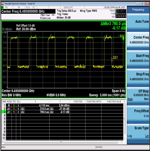
NTNV-11AX40SISO-Ant1-6485
