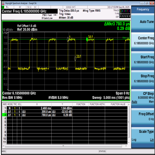
NTNV-11AX160SISO-Ant1-6185
