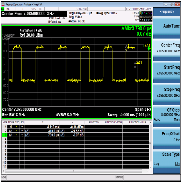
NTNV-11AX40SISO-Ant1-7085
