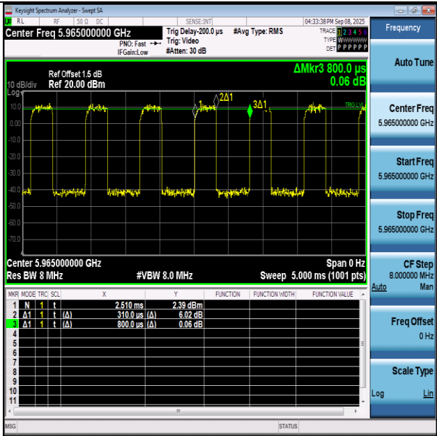
NTNV-11AX40SISO-Ant1-5965
