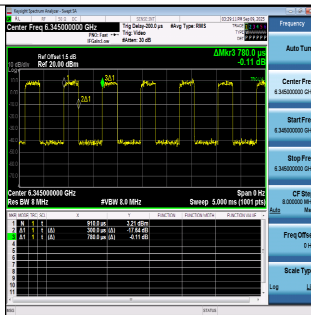
NTNV-11AX160SISO-Ant1-6345
