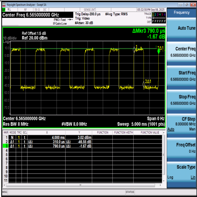
NTNV-11AX40SISO-Ant1-6565
