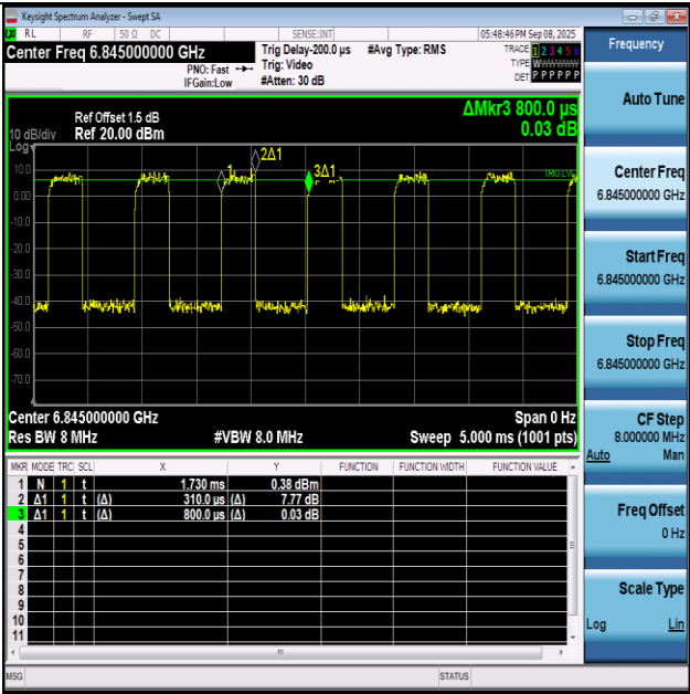
NTNV-11AX40SISO-Ant1-6845
