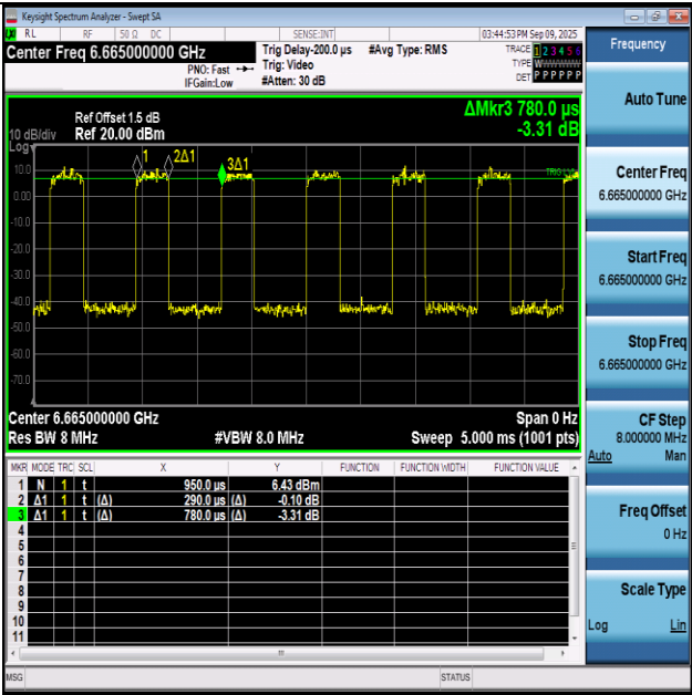
NTNV-11AX160SISO-Ant1-6665
