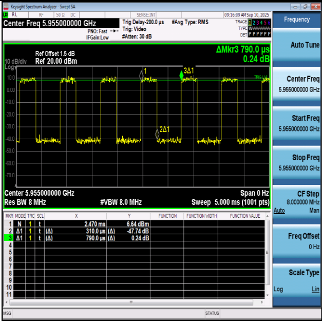
NTNV-11BE20SISO-Ant1-5955
