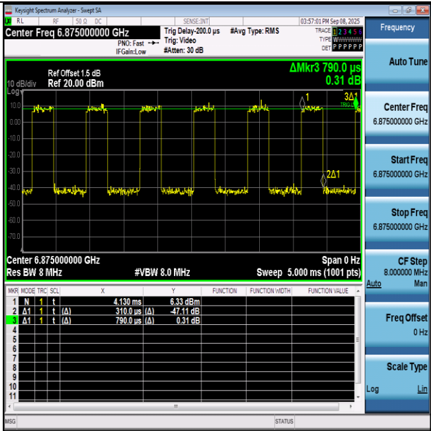
NTNV-11AX20SISO-Ant1-6875
