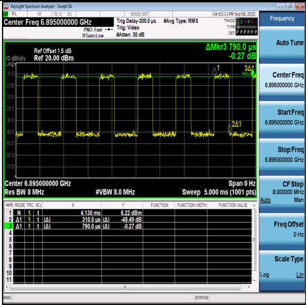
NTNV-11AX20SISO-Ant1-6895
