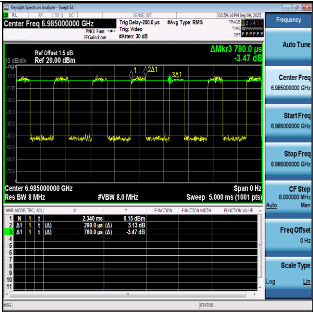
NTNV-11AX160SISO-Ant1-6985
