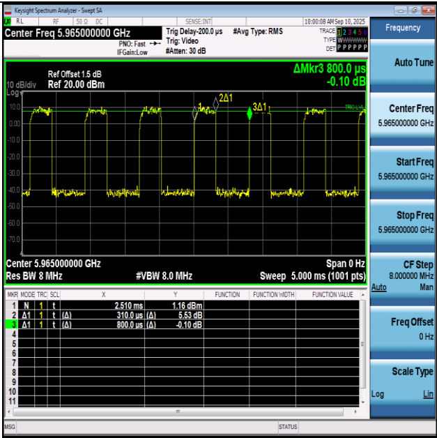
NTNV-11BE40SISO-Ant1-5965
