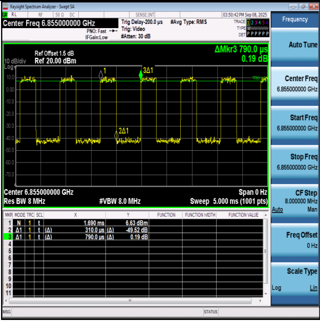
NTNV-11AX20SISO-Ant1-6855
