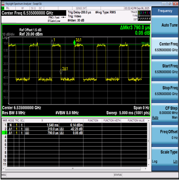
NTNV-11AX20SISO-Ant1-6535
