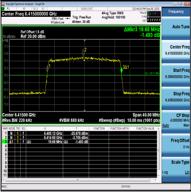
11AX20SISO-Ant1-6415
