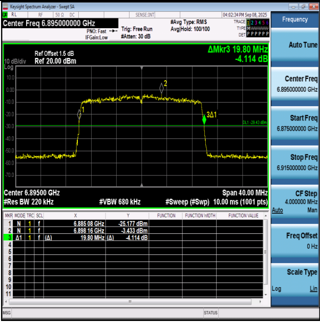
11AX20SISO-Ant1-6895
