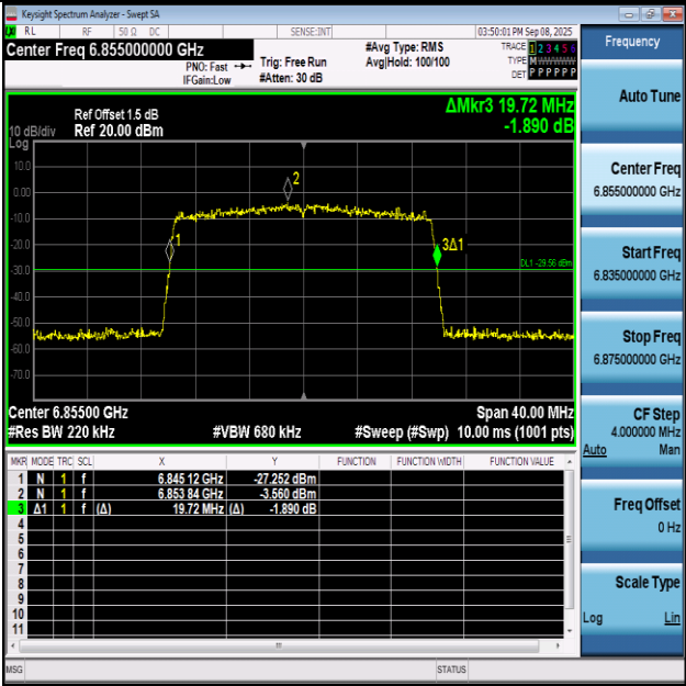
11AX20SISO-Ant1-6855
