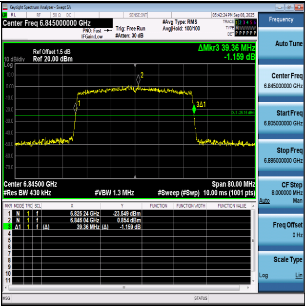
11AX40SISO-Ant1-6845
