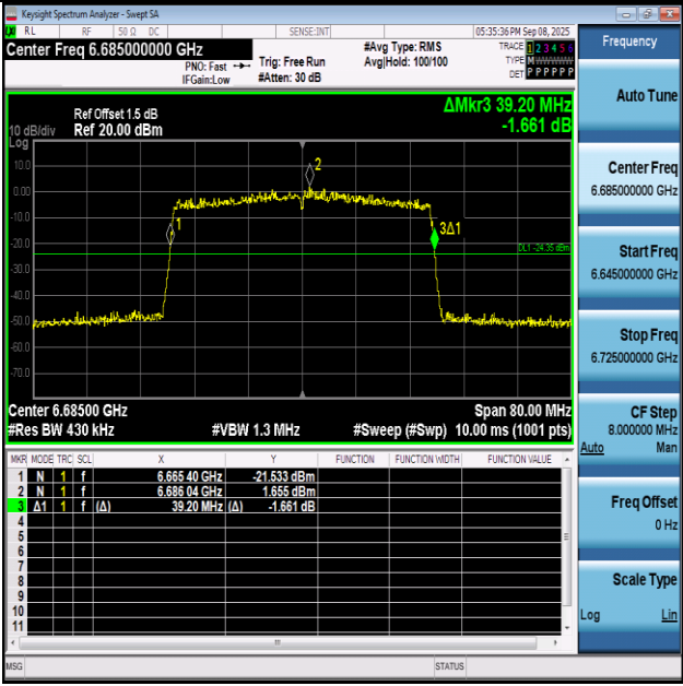
11AX40SISO-Ant1-6685
