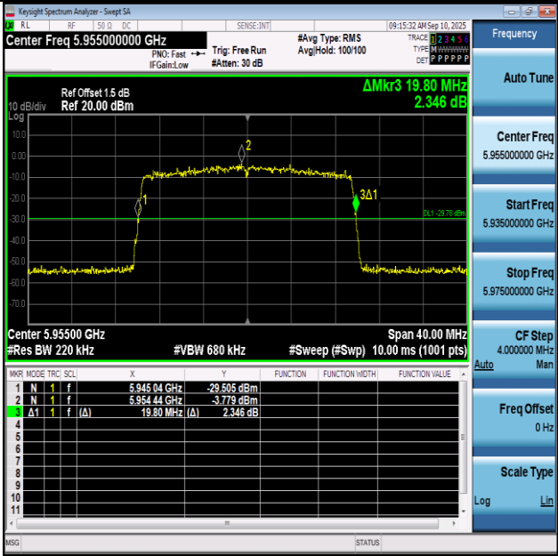
11BE20SISO-Ant1-5955
