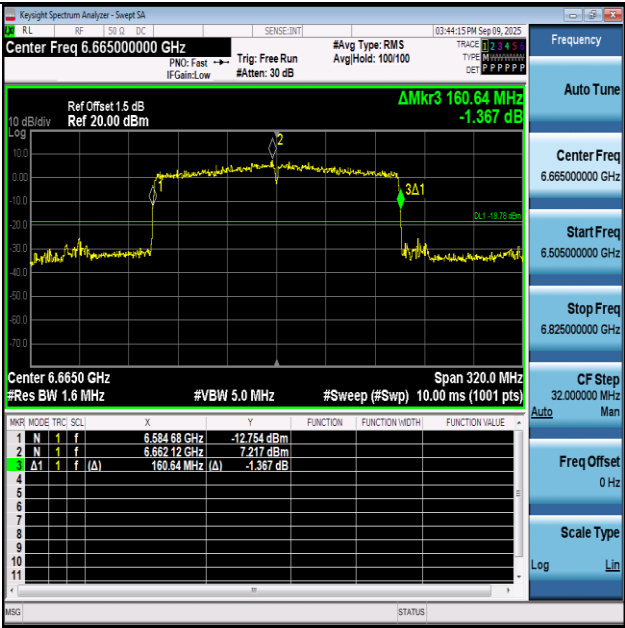
11AX160SISO-Ant1-6665
