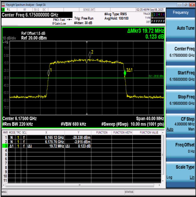
11AX20SISO-Ant1-6175
