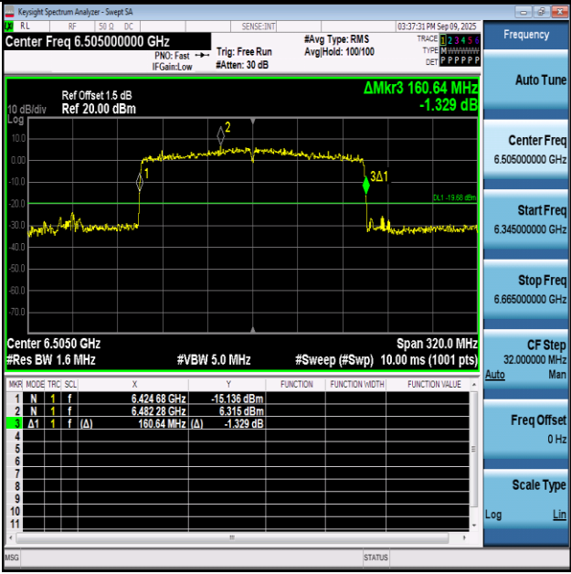
11AX160SISO-Ant1-6505
