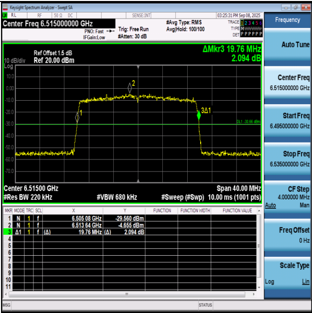
11AX20SISO-Ant1-6515
