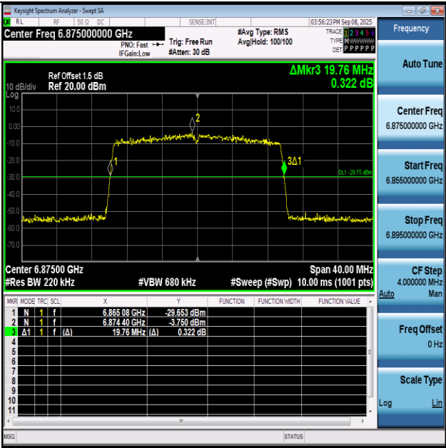
11AX20SISO-Ant1-6875
