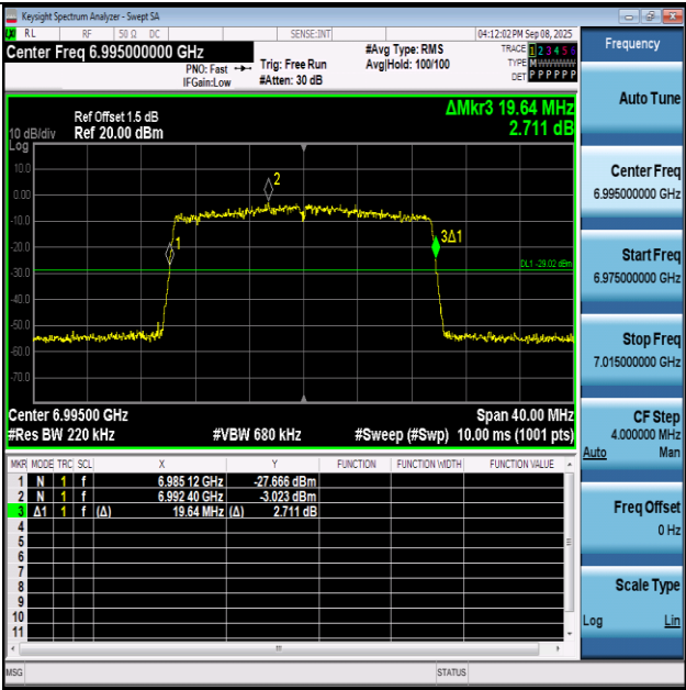
11AX20SISO-Ant1-6995
