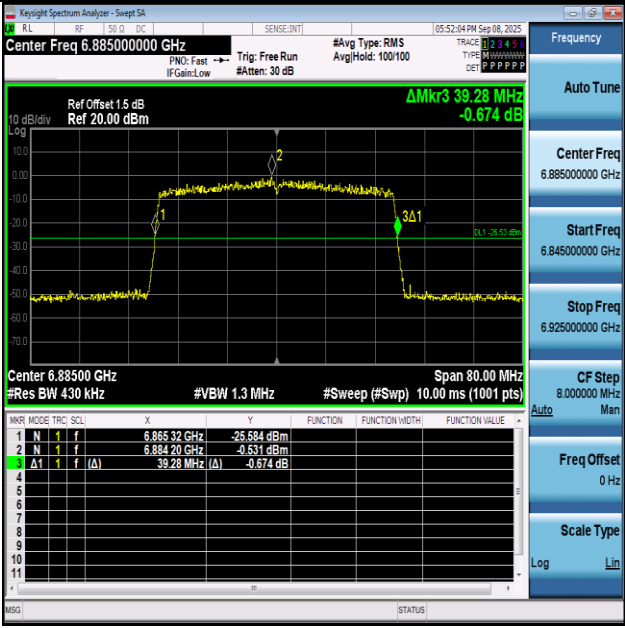
11AX40SISO-Ant1-6885
