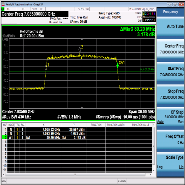
11AX40SISO-Ant1-7085
