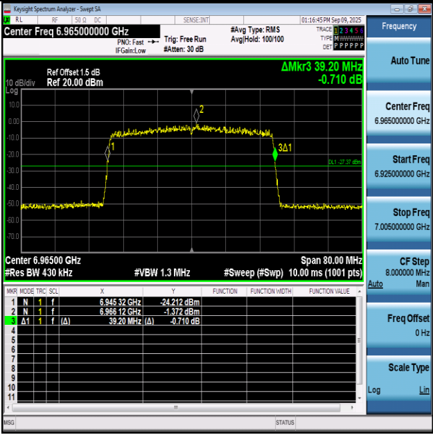
11AX40SISO-Ant1-6965
