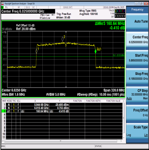
11AX160SISO-Ant1-6025
