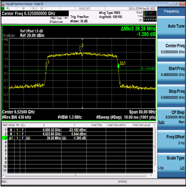
11AX40SISO-Ant1-6525
