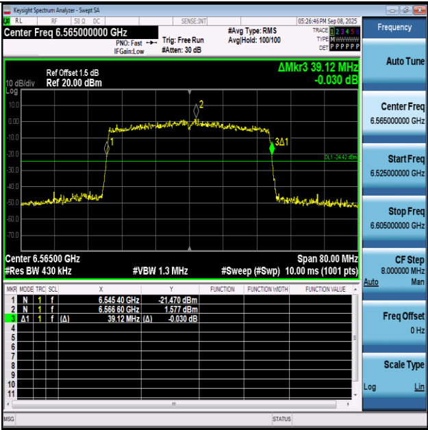
11AX40SISO-Ant1-6565
