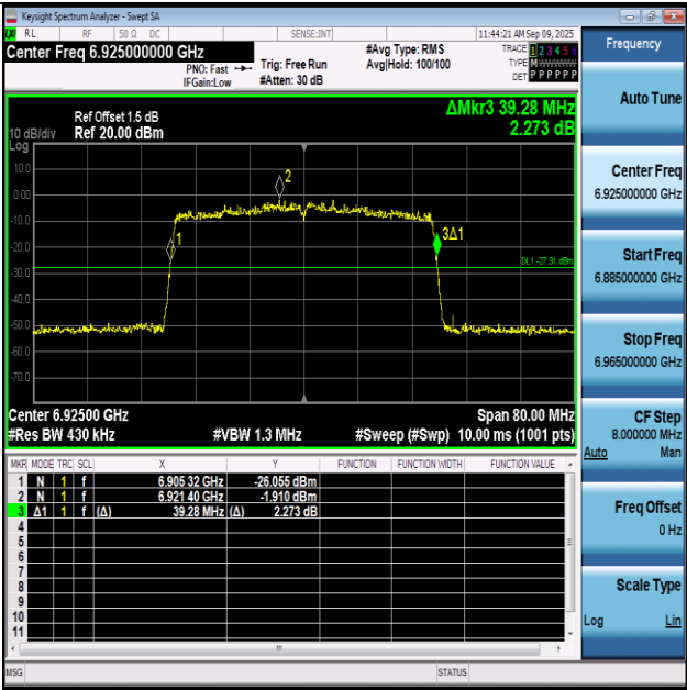
11AX40SISO-Ant1-6925
