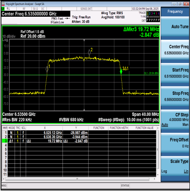
11AX20SISO-Ant1-6535
