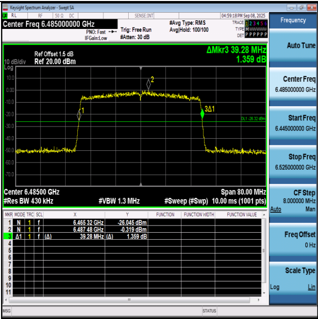
11AX40SISO-Ant1-6485
