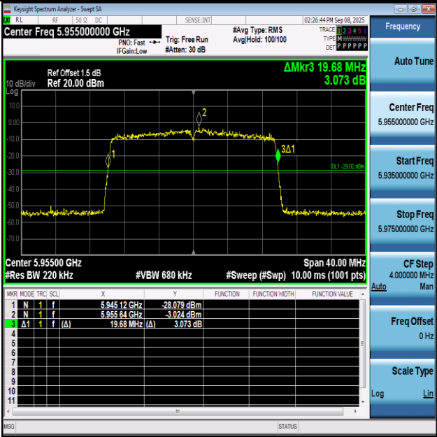
11AX20SISO-Ant1-5955
