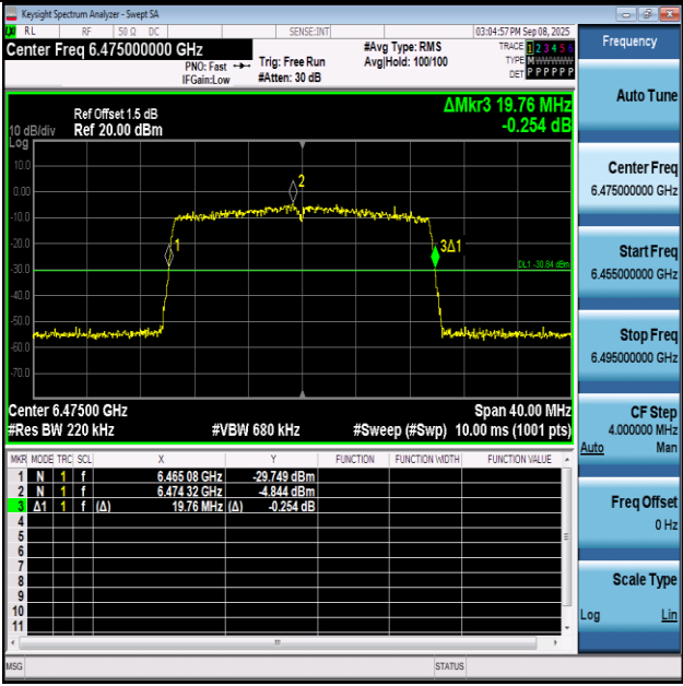
11AX20SISO-Ant1-6475
