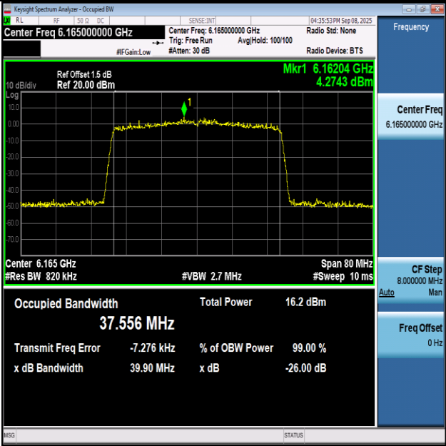
11AX40SISO-Ant1-6165-PASS
