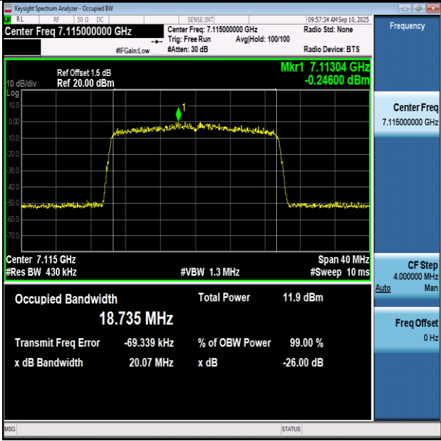
11BE20SISO-Ant1-7115-PASS
