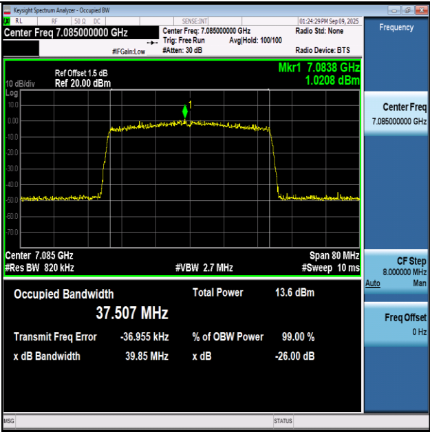
11AX40SISO-Ant1-7085-PASS
