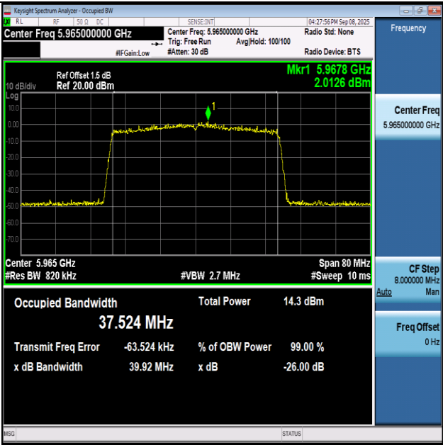
11AX40SISO-Ant1-5965-PASS
