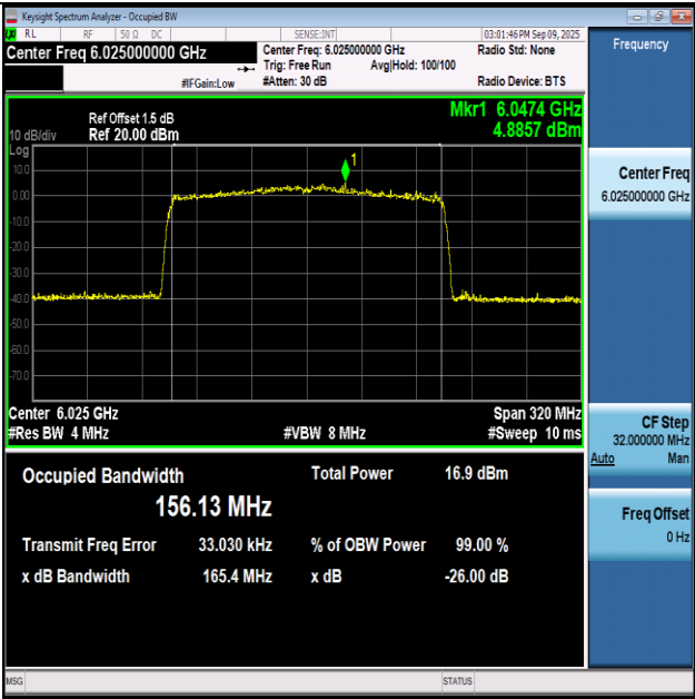
11AX160SISO-Ant1-6025-PASS
