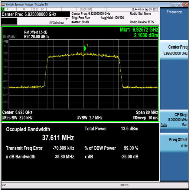
11AX40SISO-Ant1-6925-PASS
