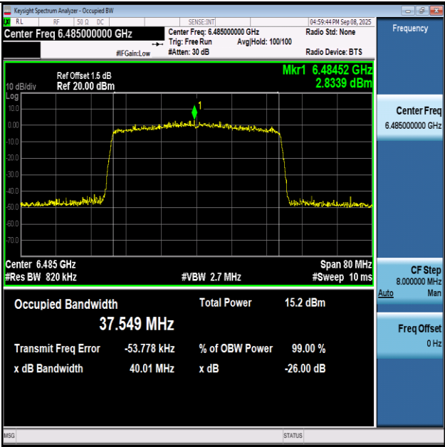
11AX40SISO-Ant1-6485-PASS
