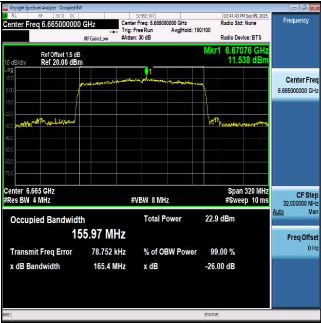
11AX160SISO-Ant1-6665-PASS
