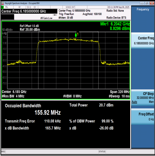
11AX160SISO-Ant1-6185-PASS
