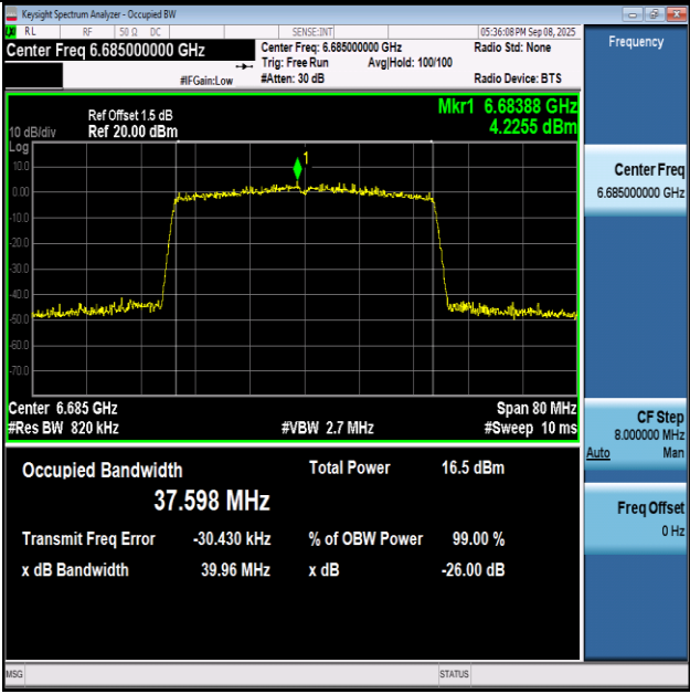
11AX40SISO-Ant1-6685-PASS
