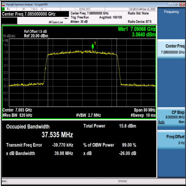
11BE40SISO-Ant1-7085-PASS
