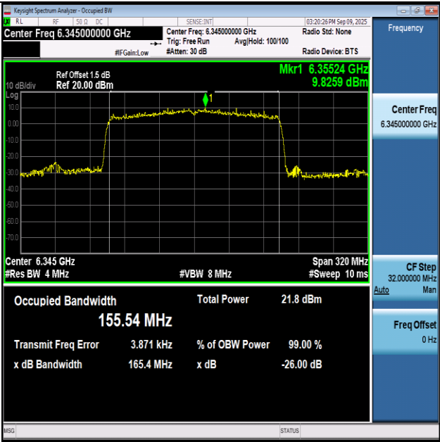
11AX160SISO-Ant1-6345-PASS
