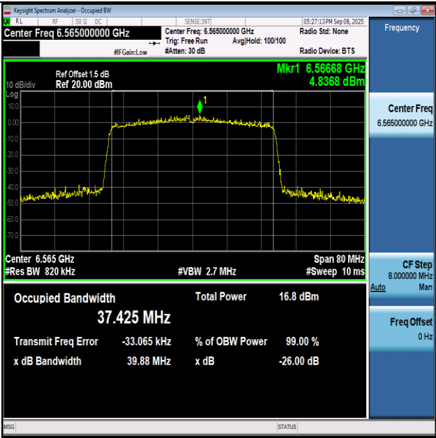
11AX40SISO-Ant1-6565-PASS
