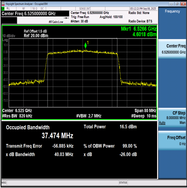
11AX40SISO-Ant1-6525-PASS
