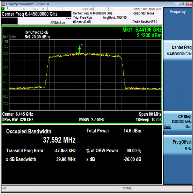
11AX40SISO-Ant1-6445-PASS
