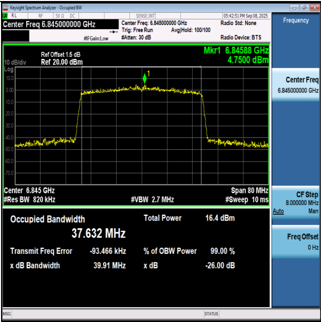
11AX40SISO-Ant1-6845-PASS
