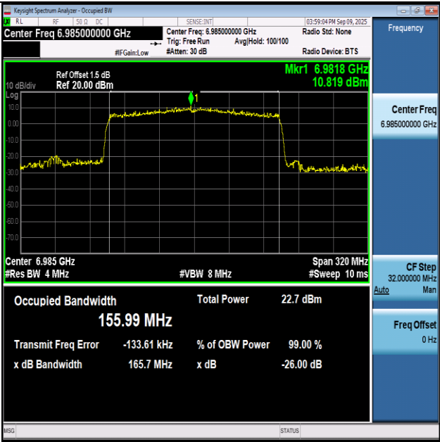
11AX160SISO-Ant1-6985-PASS
