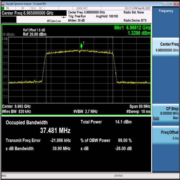
11AX40SISO-Ant1-6965-PASS
