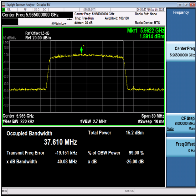
11BE40SISO-Ant1-5965-PASS
