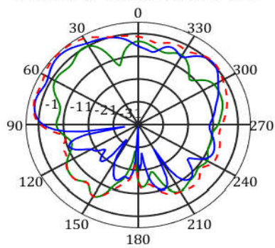
frequency=2450MHz, X-Z Plane
