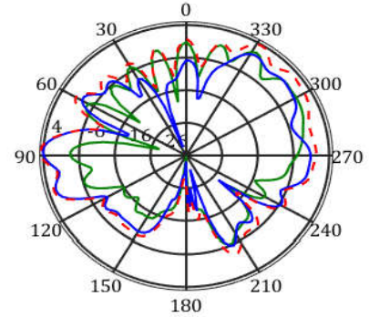
frequency=5850MHz, Y-Z Plane
