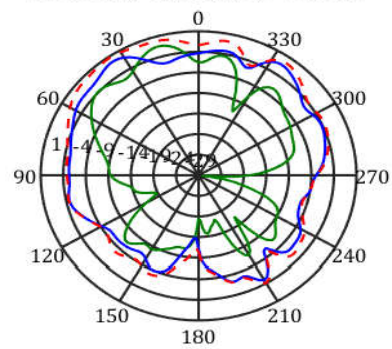
frequency=2450MHz, Y-Z Plane
