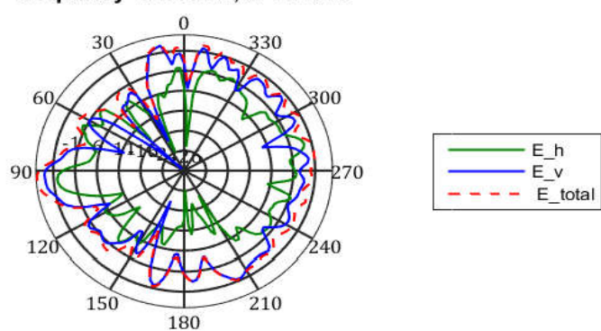
frequency=5150MHz, X-Y Plane
