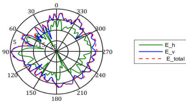
frequency=5850MHz, X-Y Plane
