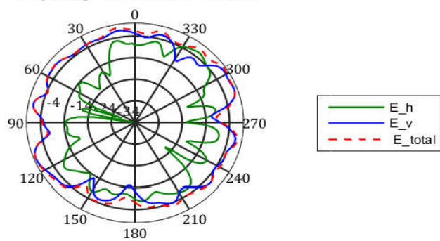
frequency=2450MHz, X-Y Plane
