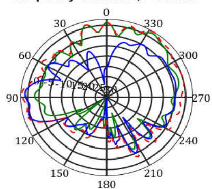
frequency=5150MHz, Y-Z Plane
