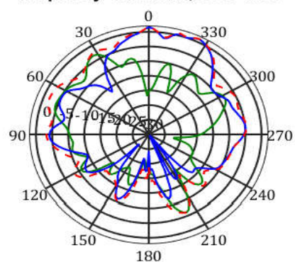
frequency=5150MHz, X-Z Plane
