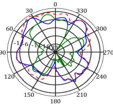
frequency=2400MHz, Y-Z Plane
