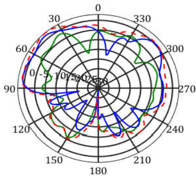
frequency=2400MHz, X-Z Plane
