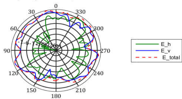
frequency=2500MHz, X-Y Plane
