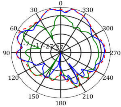
frequency=5850MHz, X-Z Plane
