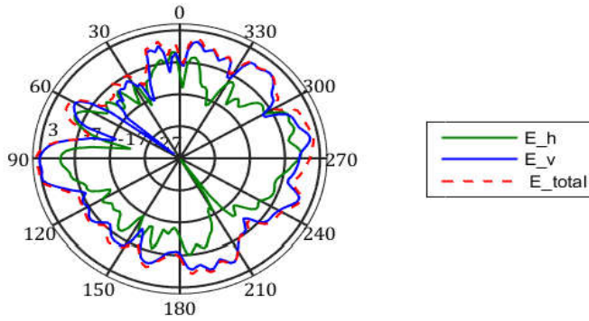
frequency=5500MHz, X-Y Plane
