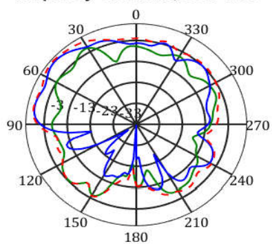
frequency=2500MHz, X-Z Plane
