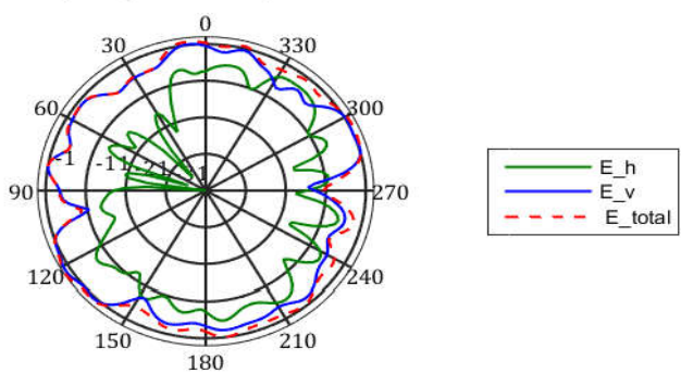
frequency=2400MHz, X-Y Plane
