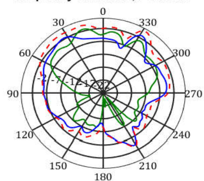
frequency=2500MHz, Y-Z Plane
