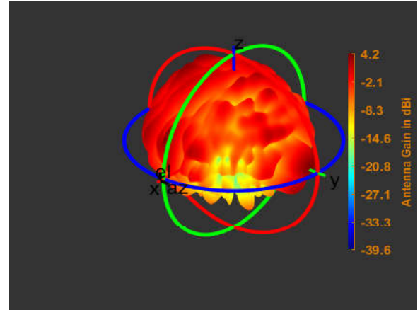
frequency=5850MHz, Y-Z Plane
