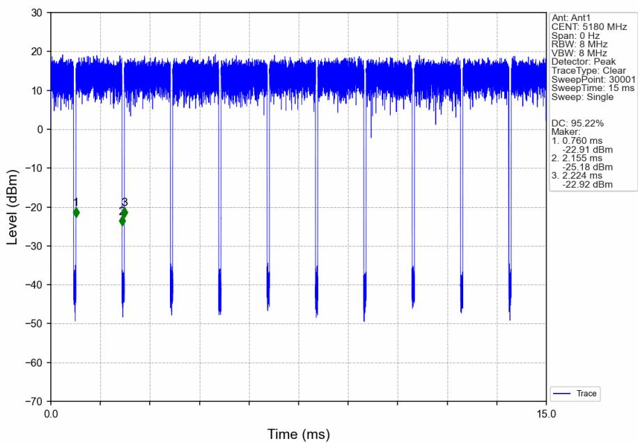
802.11a_LCH_5180MHz_Ant1_NTNV
