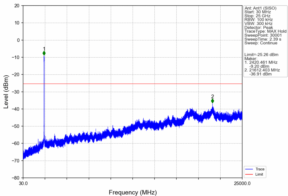
802.11n(HT40)_MCH_2437MHz_Ant1_NTNV
