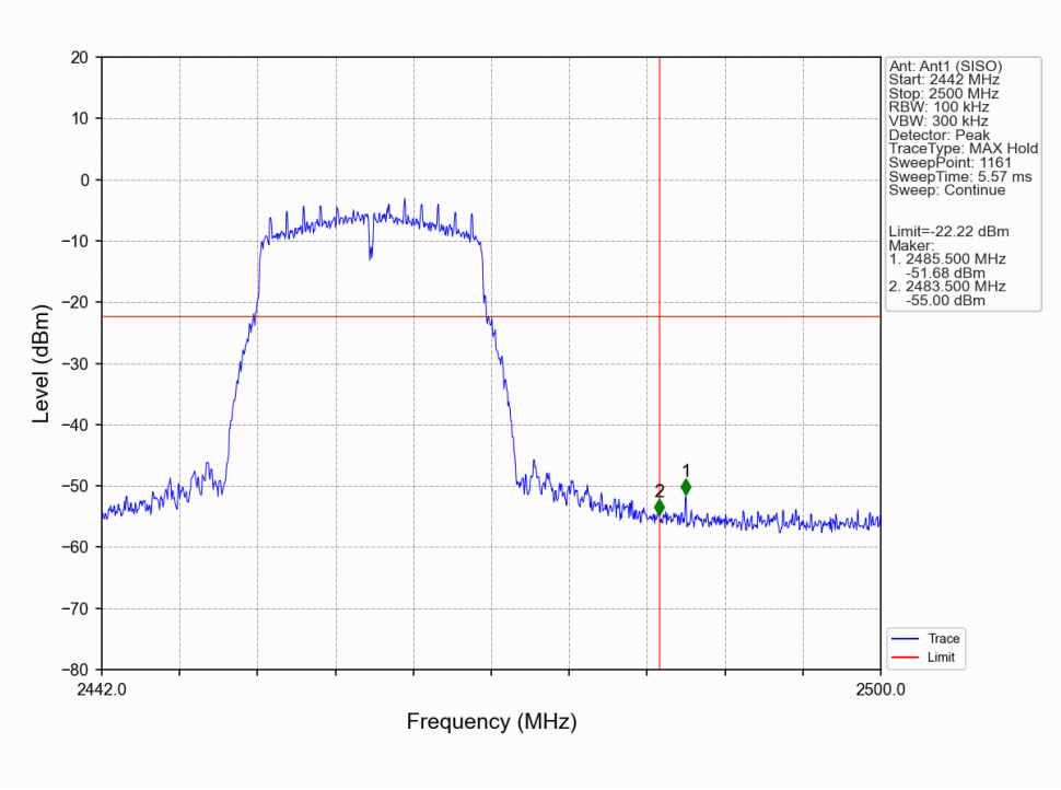
802.11g_HCH_2462MHz_Ant1_NTNV
