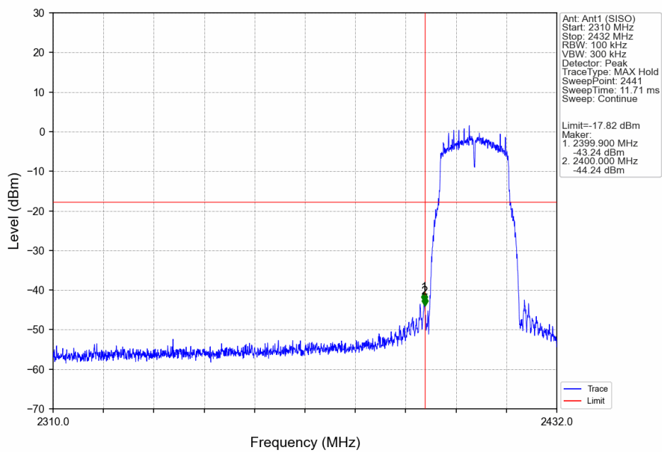
802.11g_LCH_2412MHz_Ant1_NTNV
