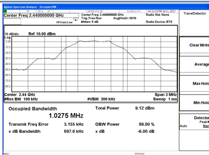
Channel 19 / 2440 MHz
