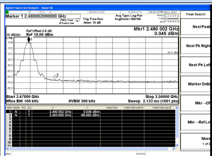
Channel 39 / 2480 MHz
