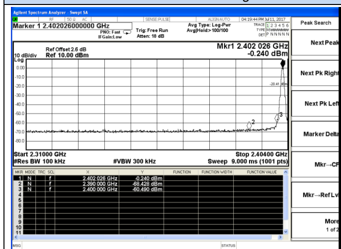
Channel 0 / 2402 MHz
