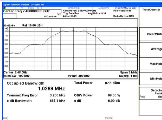
Channel 39 / 2480 MHz
