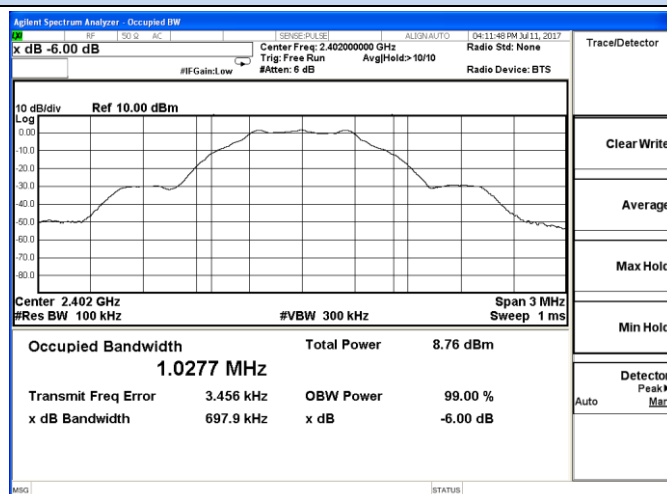
Channel 0 / 2402 MHz
