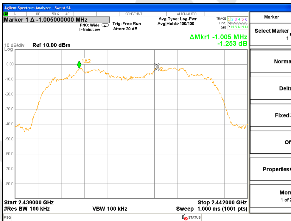
Test Mode:8DPSK---Middle
