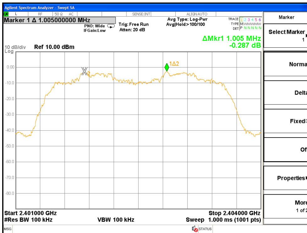
Test Mode:8DPSK---Low
