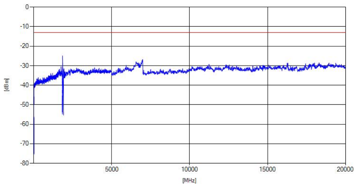
HSUPA FDD 2, Channel = low
