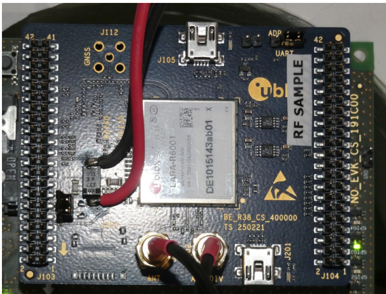
Photo 5: EUT (top side)
