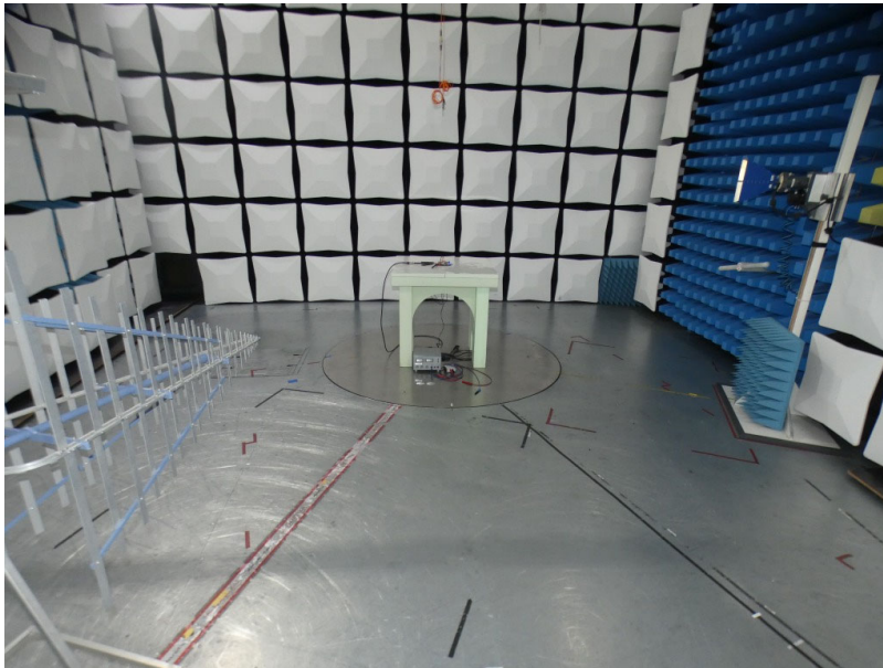
Photo 4: Test setup for radiated measurements below 1GHz
