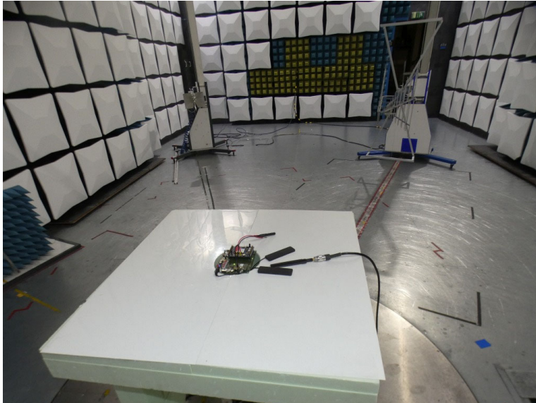
Photo 6: Test Antenna
