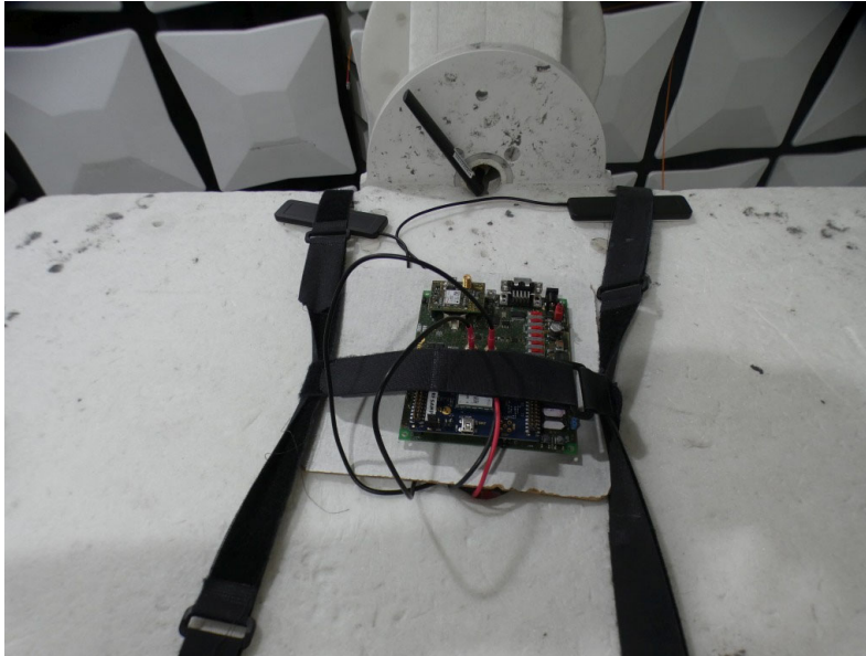
Photo 2: EUT setup
