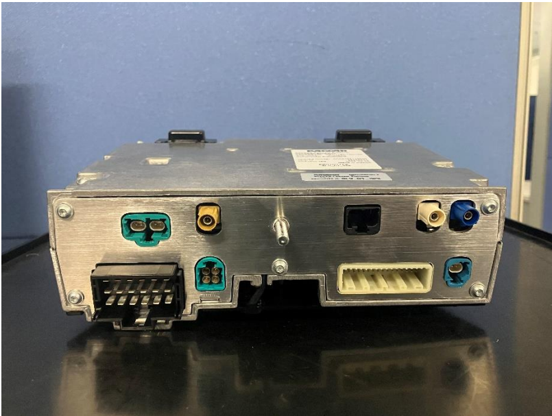
Figure 1.3 Silverbox Rear and Connectors View
