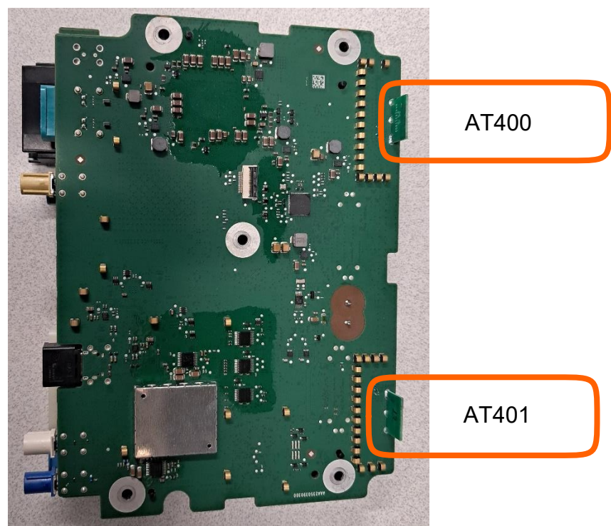
Figure 1.4 Radio PCB Bottom View
