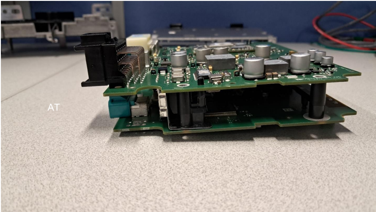
Figure 1.10 Silverbox Left side view
