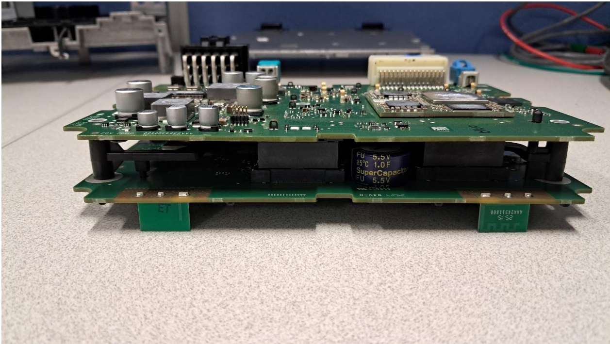
Figure 1.11 Silverbox back view
