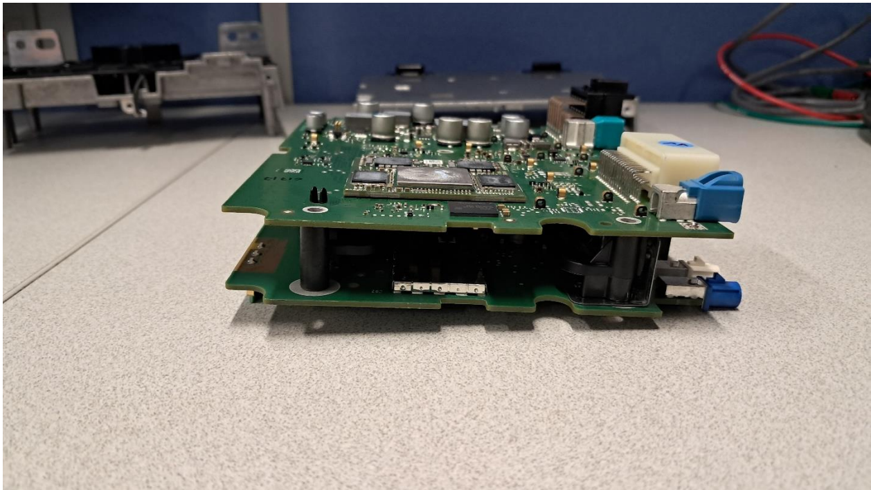
Figure 1.9 Silverbox Right side view
