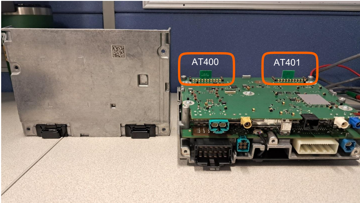
Figure 1.6 Silverbox bottom housing
