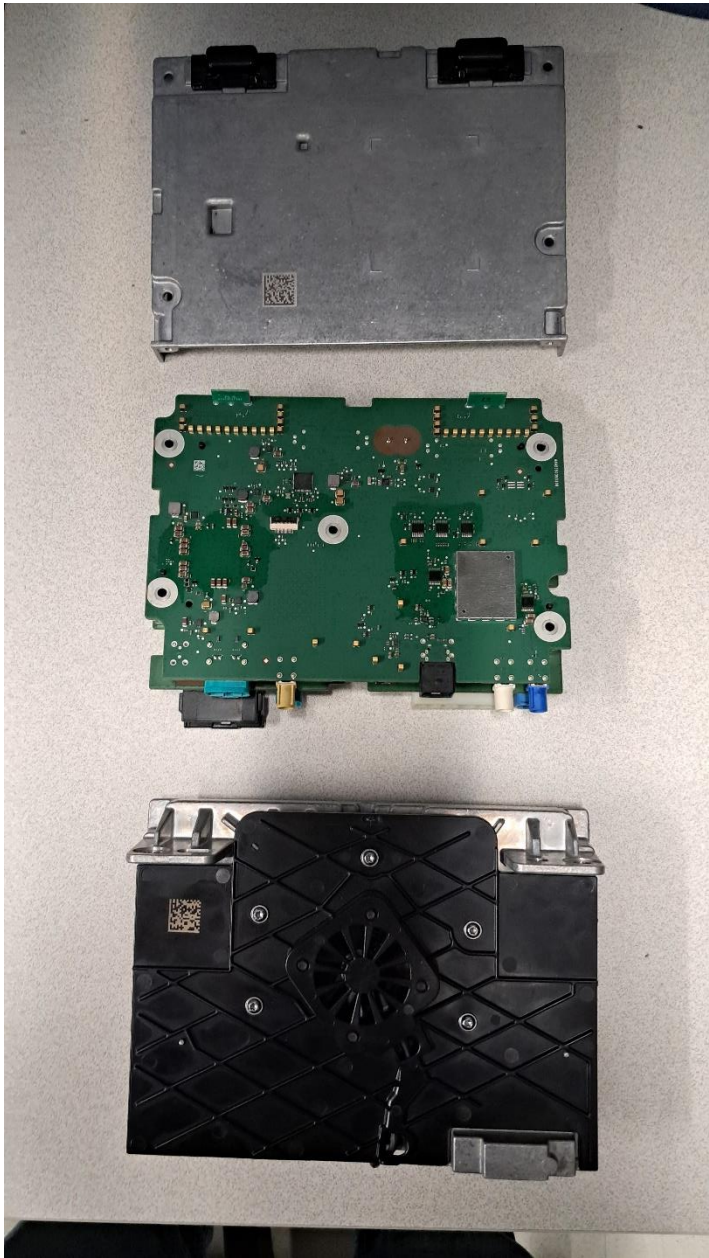
Figure 1.7 Silverbox bottom housing and top housing disassemble
