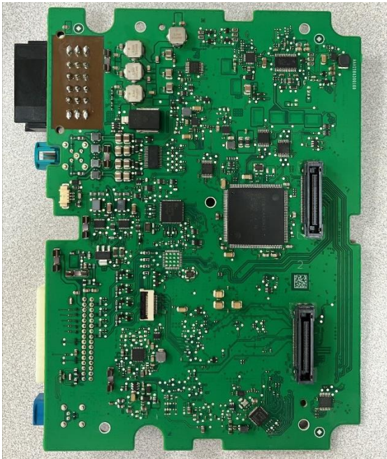
Figure 1.2 Main PCB Bottom View
