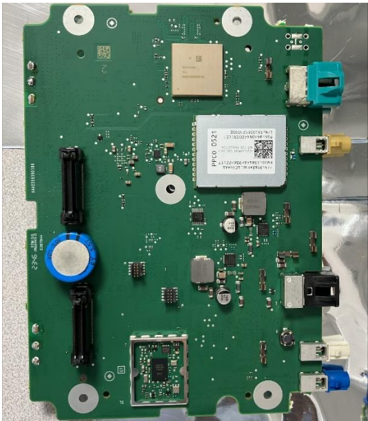
Figure 1.3 Radio PCB Top View
