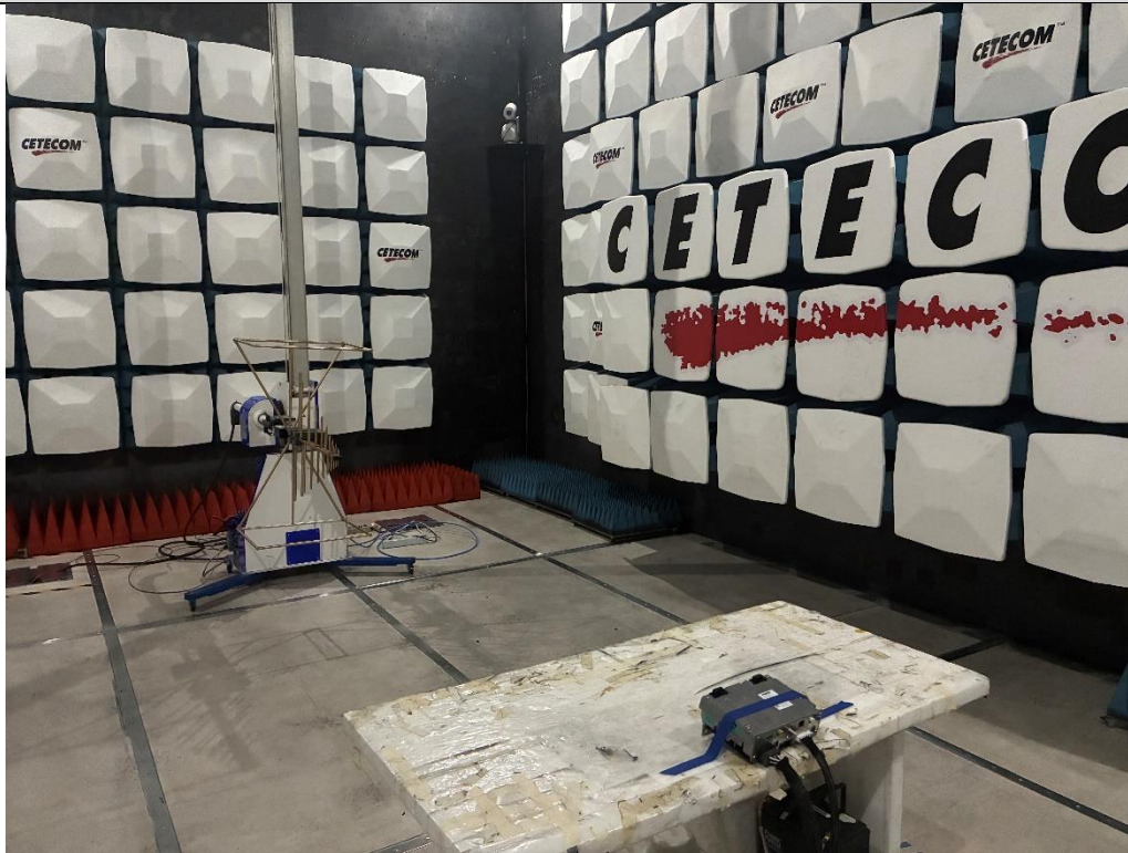
30MHz – 1GHz Rear View
