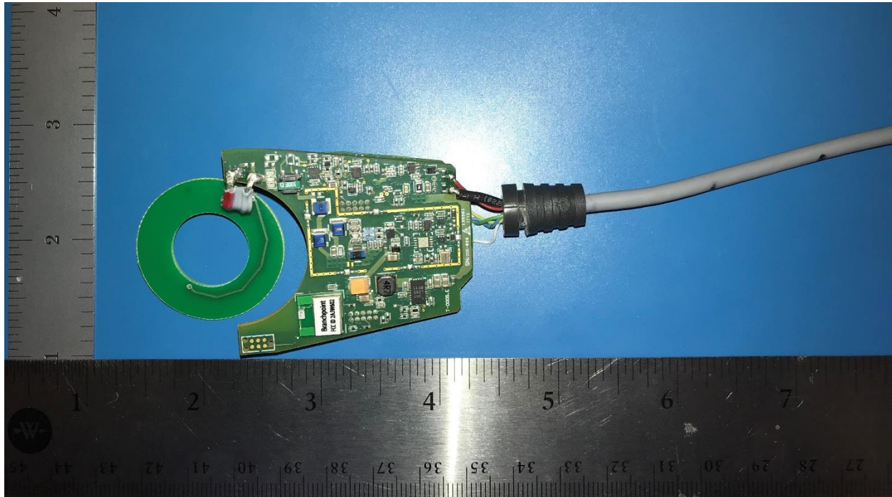
Figure 1 - AURA Monitor Antenna Interior Top
