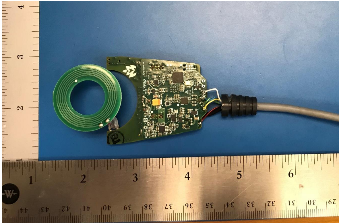
Figure 2 - AURA Monitor Antenna Interior Bottom
