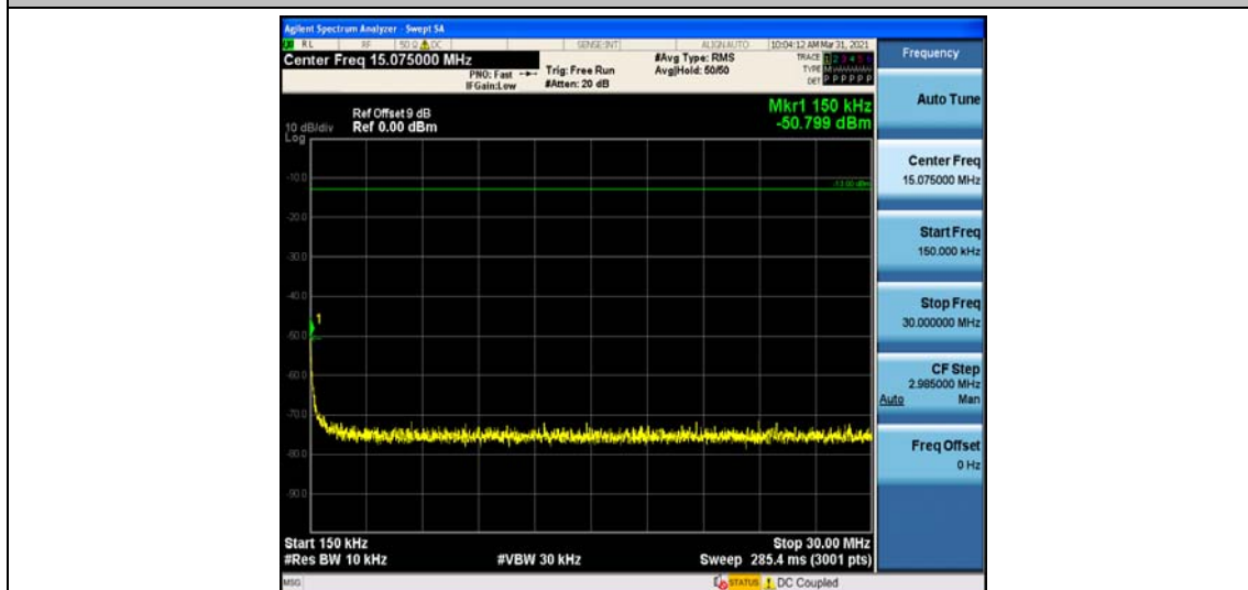
Band25_1.4MHz_16QAM_26365_1RB#0
