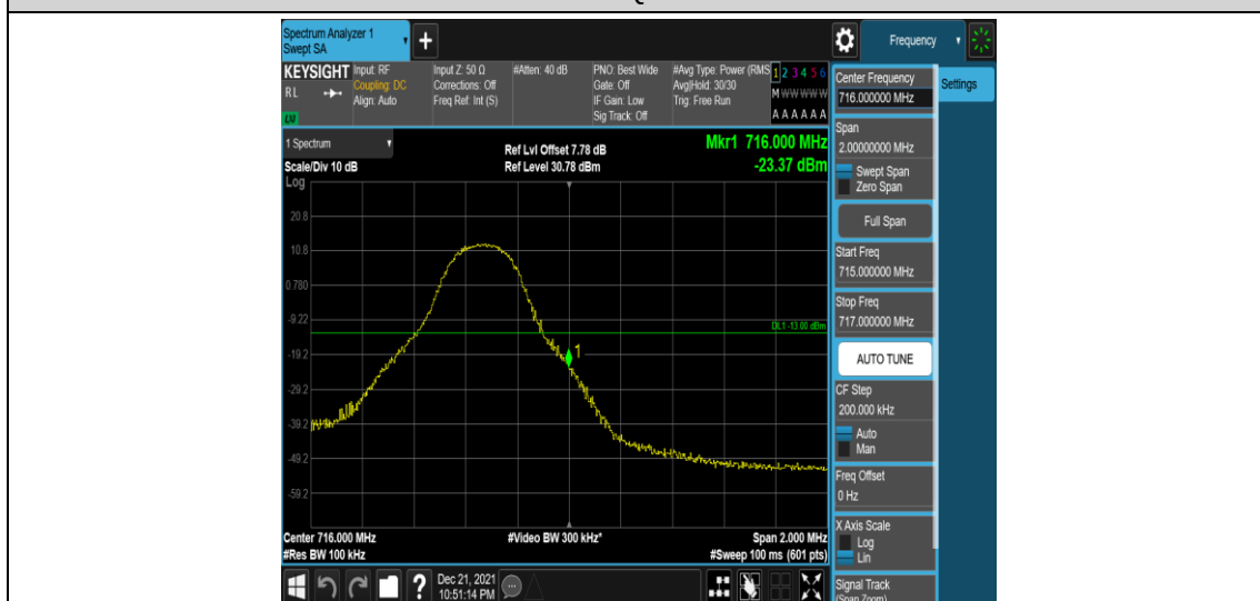
Band12-5MHz-16QAM-23155-1RB#24
