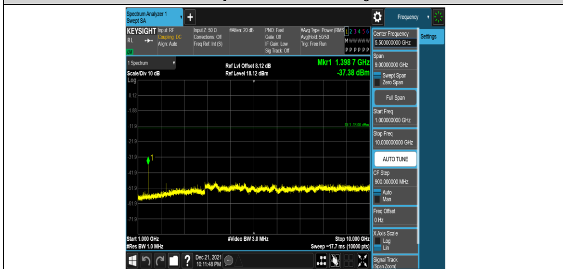
Band12-1.4MHz-16QAM-23017-1RB#0-Range4:1000~10000MHz
