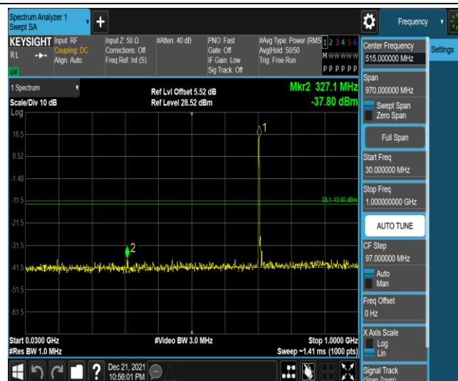
Band12-5MHz-QPSK-23155-1RB#0-Range3:30~1000MHz
