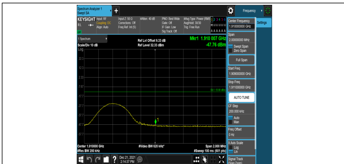
Band2-10MHz-16QAM-19150-1RB#0
