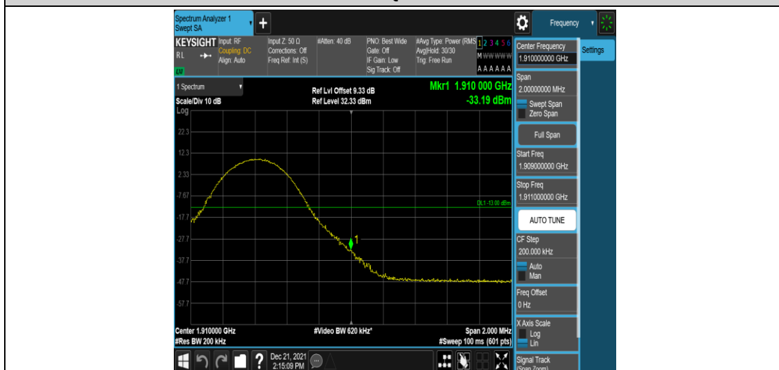
Band2-10MHz-16QAM-19150-1RB#49
