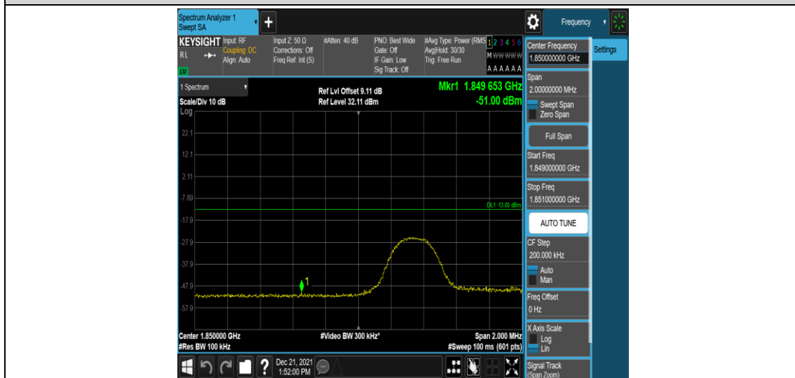
Band2-5MHz-16QAM-18625-1RB#24
