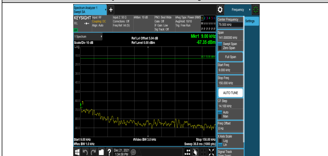
Band2-3MHz-QPSK-18900-1RB#0-Range1:0.009~0.15MHz
