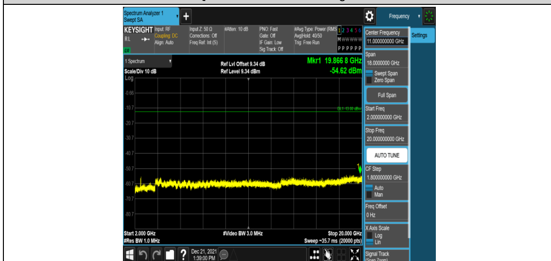
Band2-3MHz-16QAM-19185-1RB#0-Range5:2000~20000MHz
