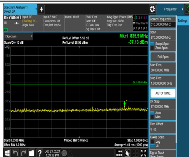
Band2-5MHz-QPSK-19175-1RB#0-Range3:30~1000MHz
