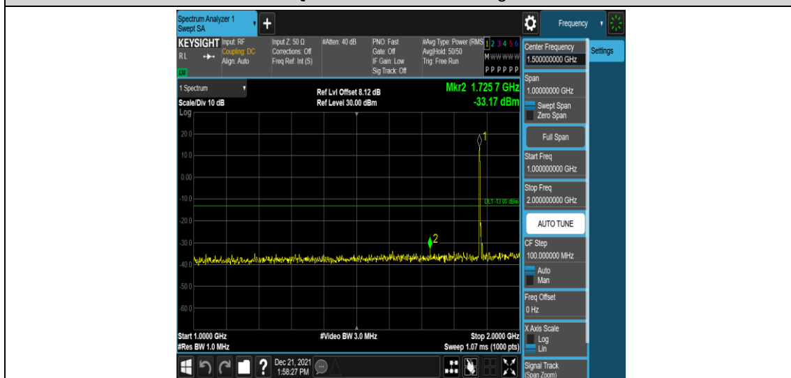
Band2-5MHz-16QAM-18900-1RB#0-Range4:1000~2000MHz
