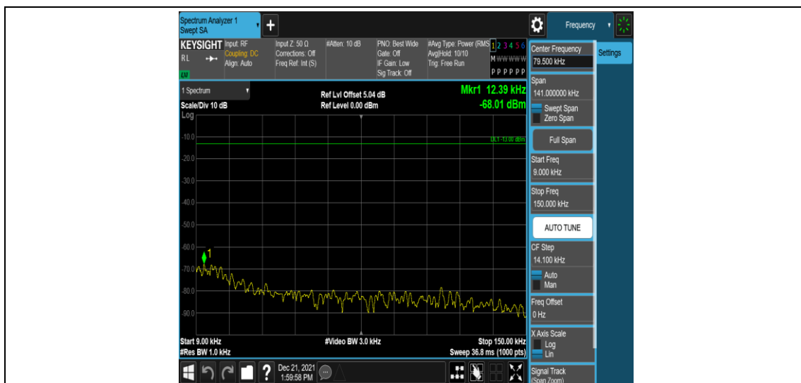
Band2-5MHz-16QAM-19175-1RB#0-Range1:0.009~0.15MHz
