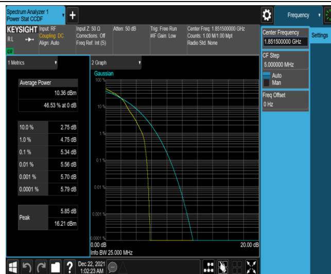
Band25-3MHz-16QAM-26055-1RB#0
