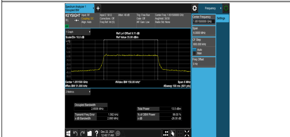
Band25-3MHz-QPSK-26055-15RB#0
