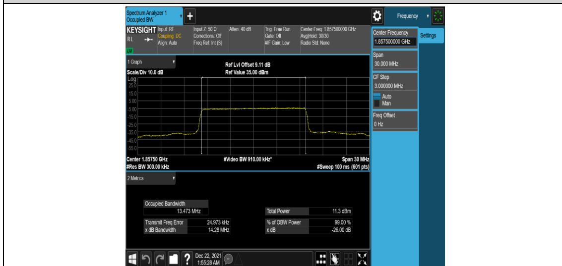
Band25-15MHz-16QAM-26115-75RB#0
