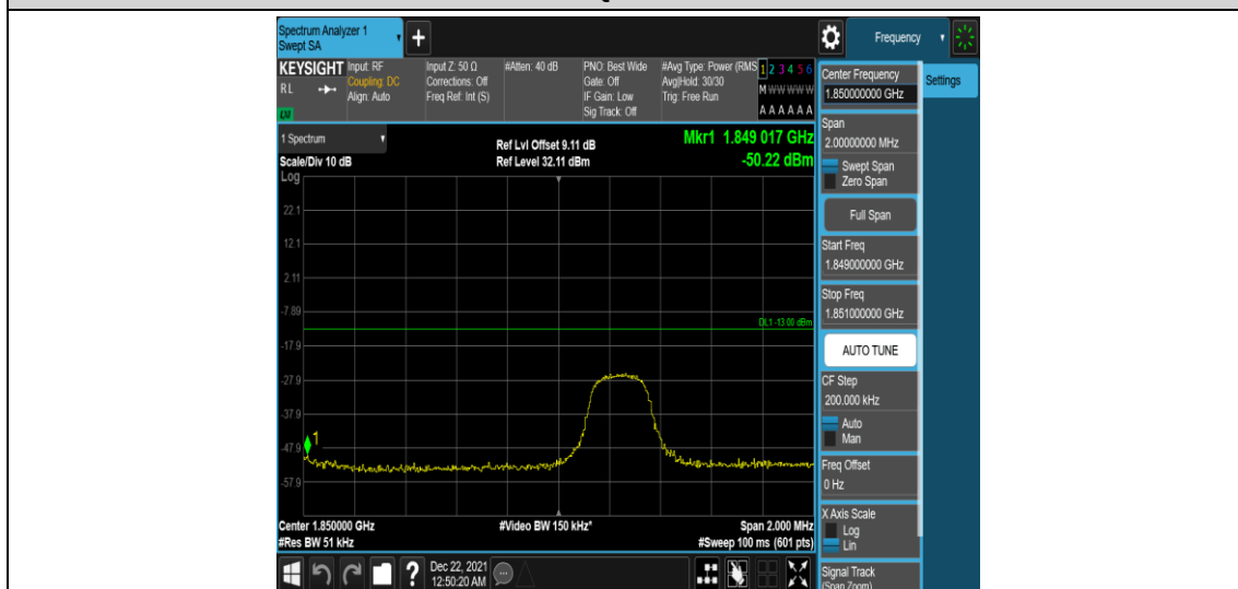
Band25-3MHz-QPSK-26055-1RB#14
