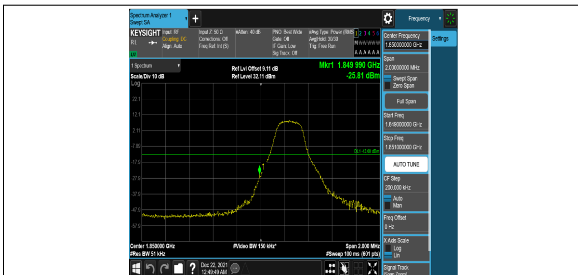
Band25-3MHz-QPSK-26055-1RB#0
