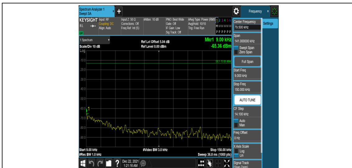
Band25-5MHz-16QAM-26665-1RB#0-Range1:0.009~0.15MHz
