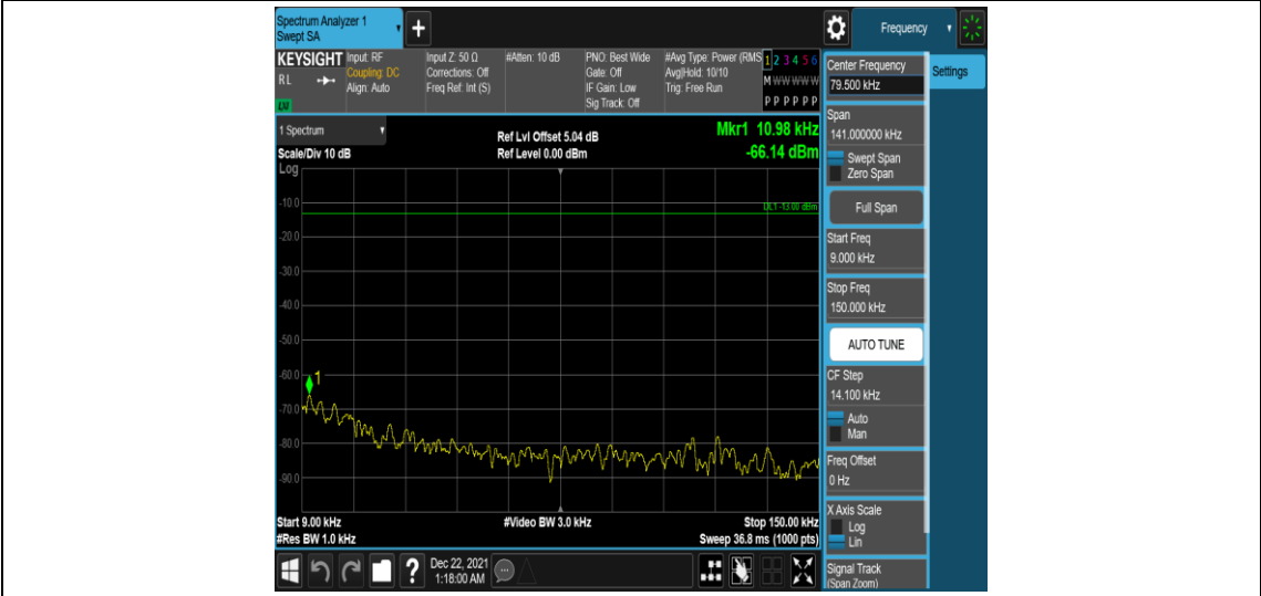
Band25-5MHz-QPSK-26365-1RB#0-Range1:0.009~0.15MHz
