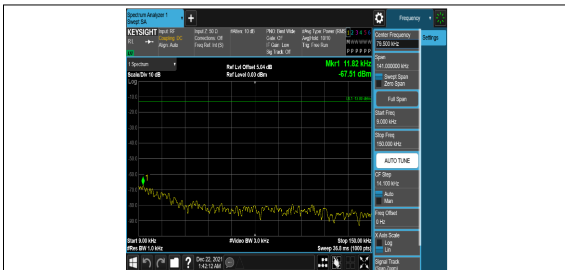
Band25-10MHz-QPSK-26640-1RB#0-Range1:0.009~0.15MHz
