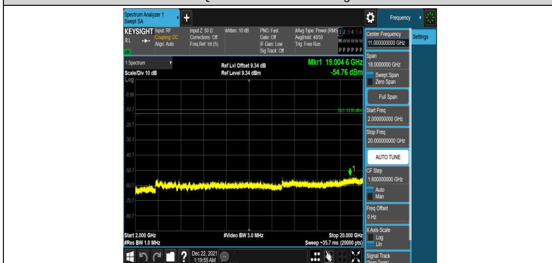
Band25-5MHz-16QAM-26365-1RB#0-Range5:2000~20000MHz
