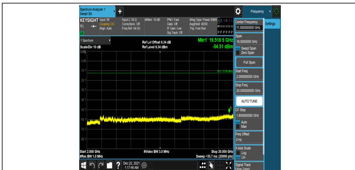
Band25-5MHz-16QAM-26065-1RB#0-Range5:2000~20000MHz
