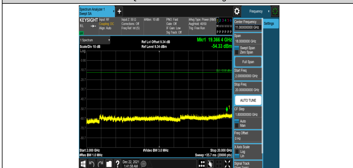
Band25-10MHz-16QAM-26365-1RB#0-Range5:2000~20000MHz
