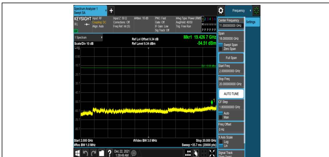
Band25-10MHz-16QAM-26090-1RB#0-Range5:2000~20000MHz
