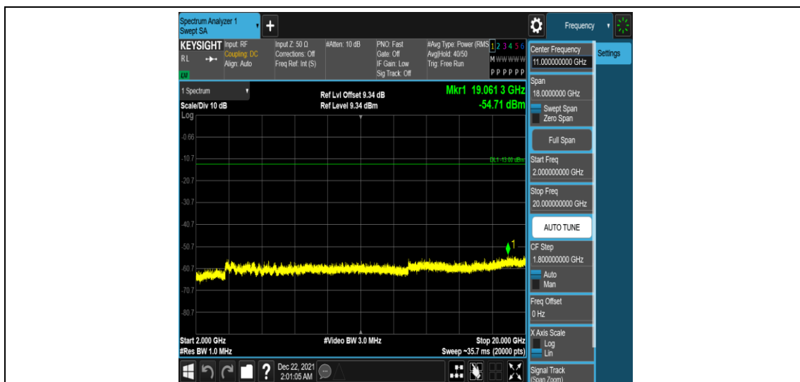
Band25-15MHz-QPSK-26115-1RB#0-Range5:2000~20000MHz
