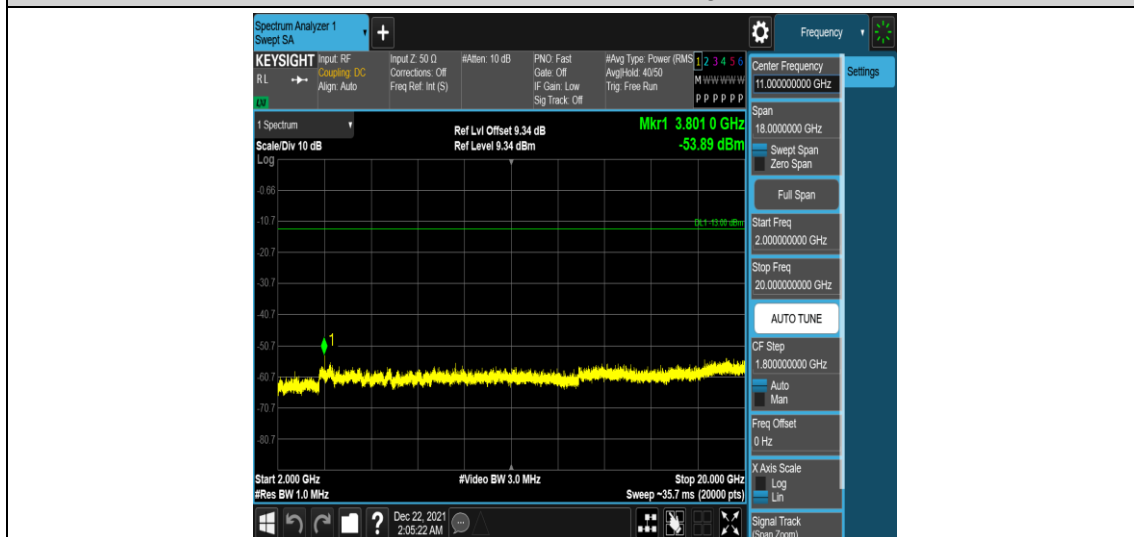
Band25-15MHz-QPSK-26615-1RB#0-Range5:2000~20000MHz
