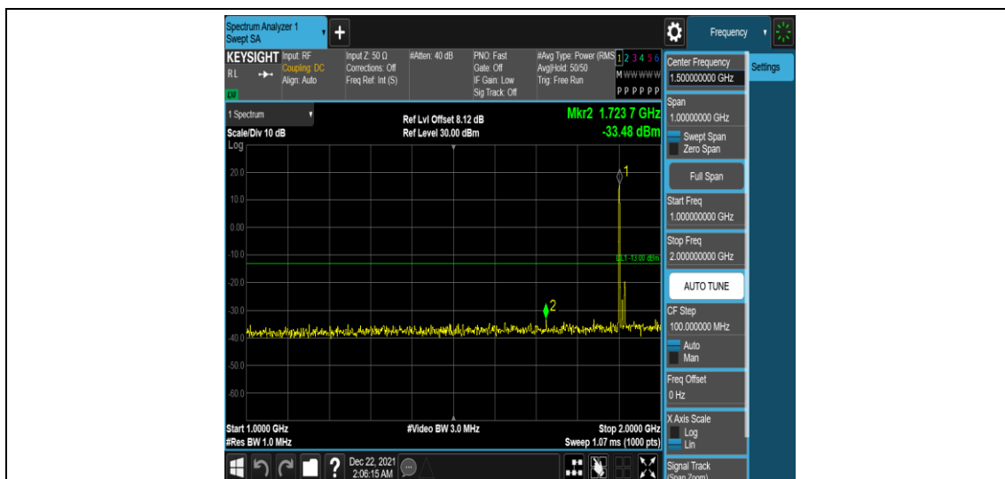
Band25-15MHz-16QAM-26615-1RB#0-Range4:1000~2000MHz
