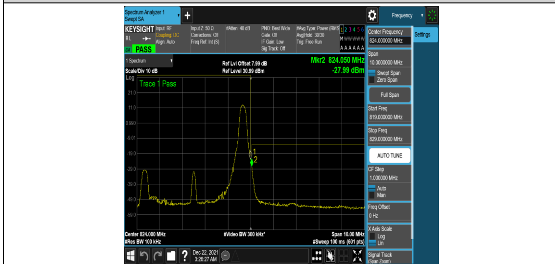
Band26-5MHz-QPSK-26765-1RB#24
