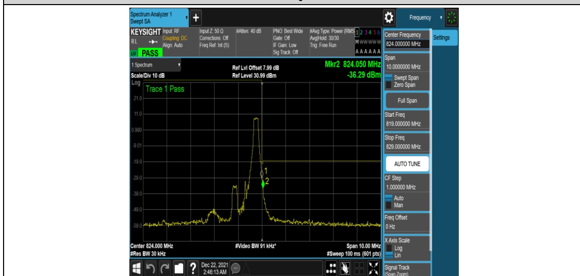
Band26-1.4MHz-16QAM-26783-1RB#5
