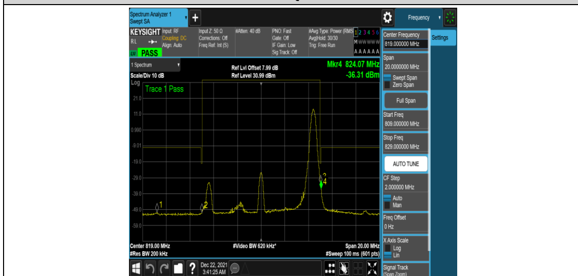
Band26-10MHz-16QAM-26740-1RB#49
