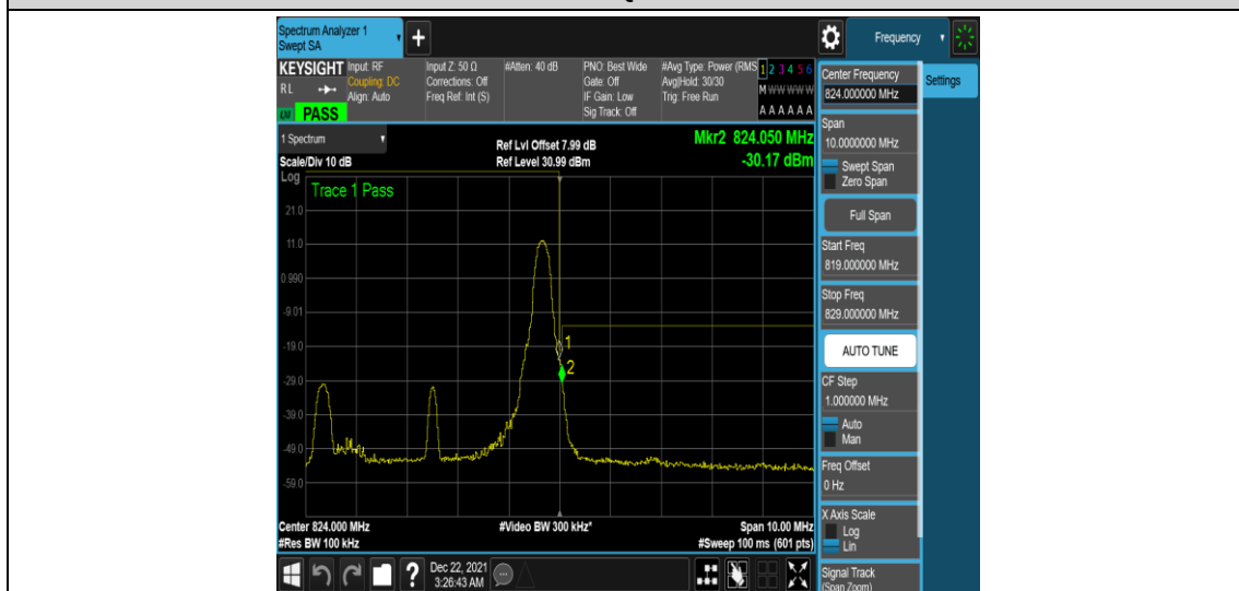
Band26-5MHz-16QAM-26765-1RB#24
