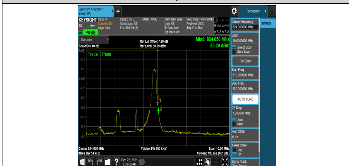
Band26-3MHz-16QAM-26775-1RB#14
