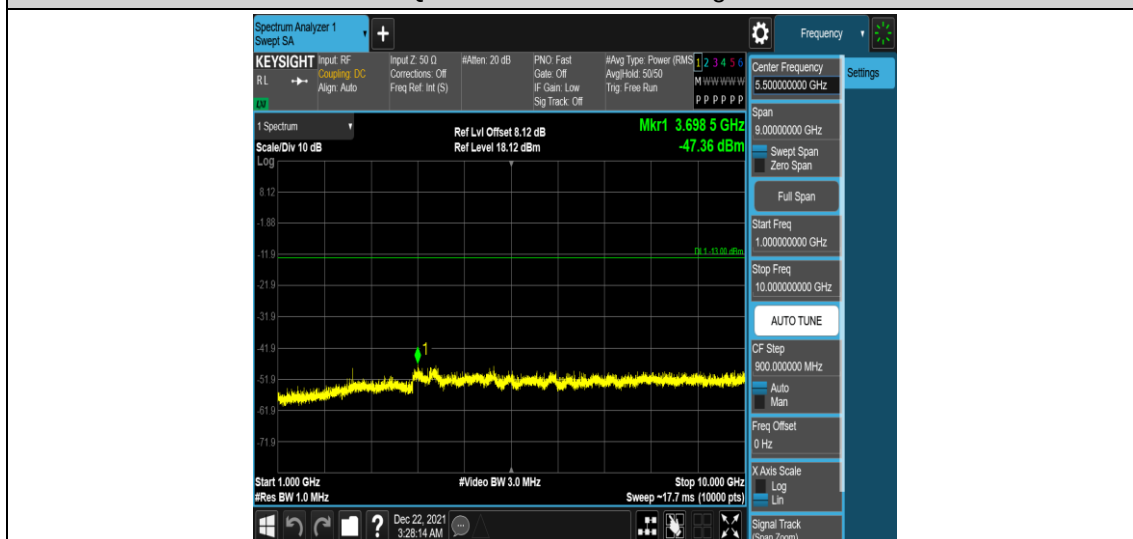
Band26-5MHz-QPSK-26715-1RB#0-Range4:1000~10000MHz
