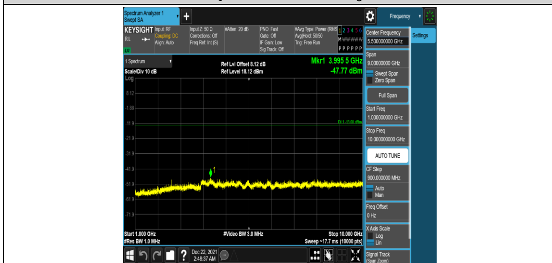
Band26-1.4MHz-16QAM-26697-1RB#0-Range4:1000~10000MHz
