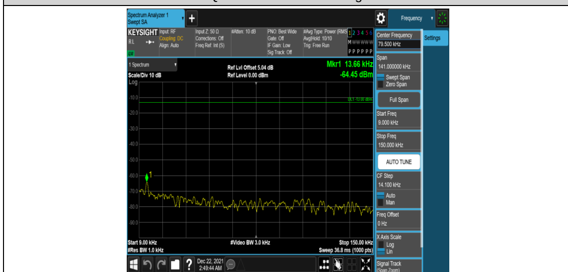
Band26-1.4MHz-16QAM-26740-1RB#0-Range1:0.009~0.15MHz
