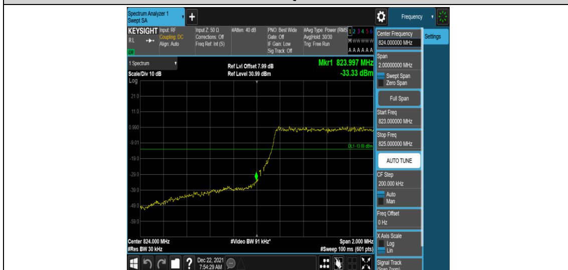
Band26-1.4MHz-16QAM-26797-6RB#0
