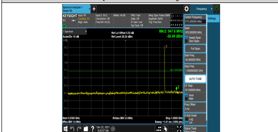
Band26-3MHz-QPSK-27025-1RB#0-Range3:30~1000MHz
