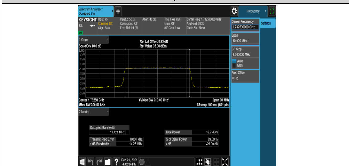
Band4-15MHz-16QAM-20175-75RB#0
