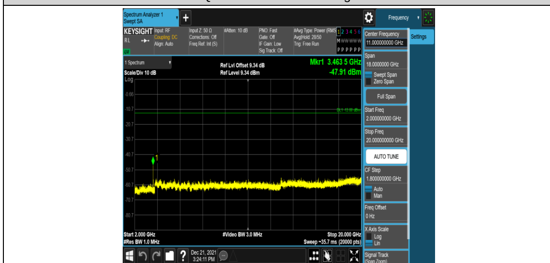
Band4-1.4MHz-16QAM-20175-1RB#0-Range5:2000~20000MHz
