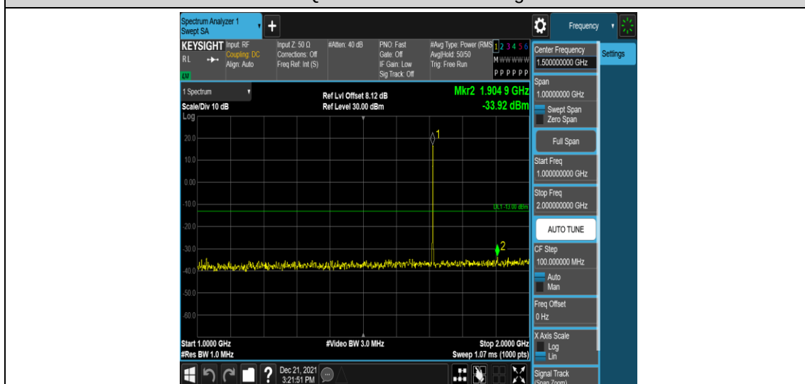
Band4-1.4MHz-16QAM-19957-1RB#0-Range4:1000~2000MHz
