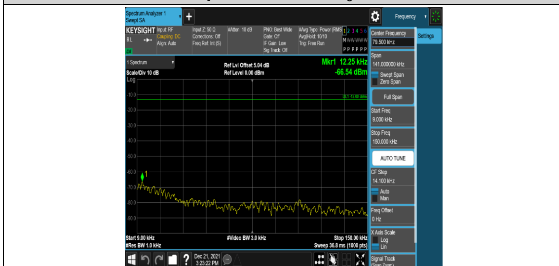
Band4-1.4MHz-16QAM-20175-1RB#0-Range1:0.009~0.15MHz
