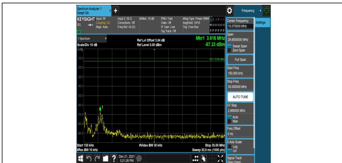
Band4-1.4MHz-16QAM-19957-1RB#0-Range2:0.15~30MHz
