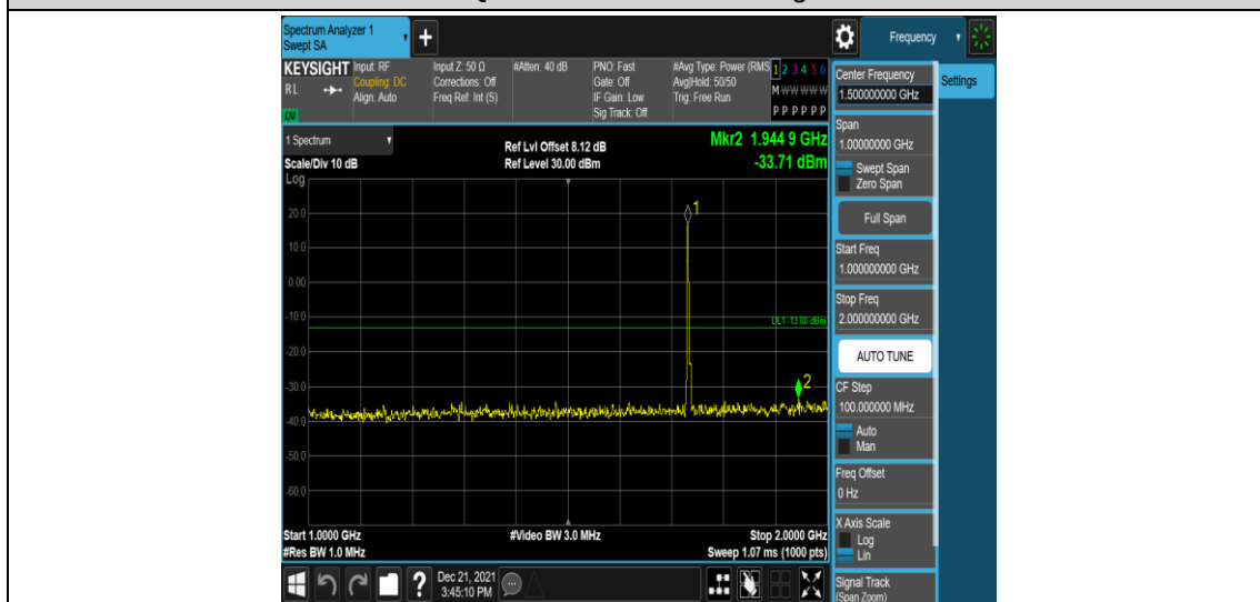
Band4-3MHz-16QAM-20175-1RB#0-Range4:1000~2000MHz
