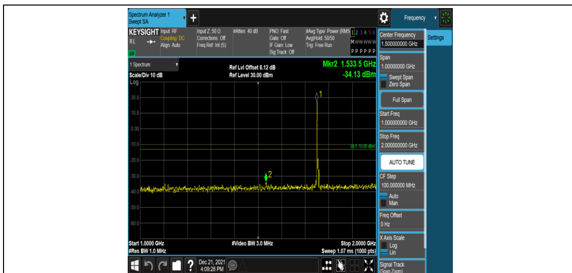
Band4-5MHz-16QAM-20375-1RB#0-Range4:1000~2000MHz
