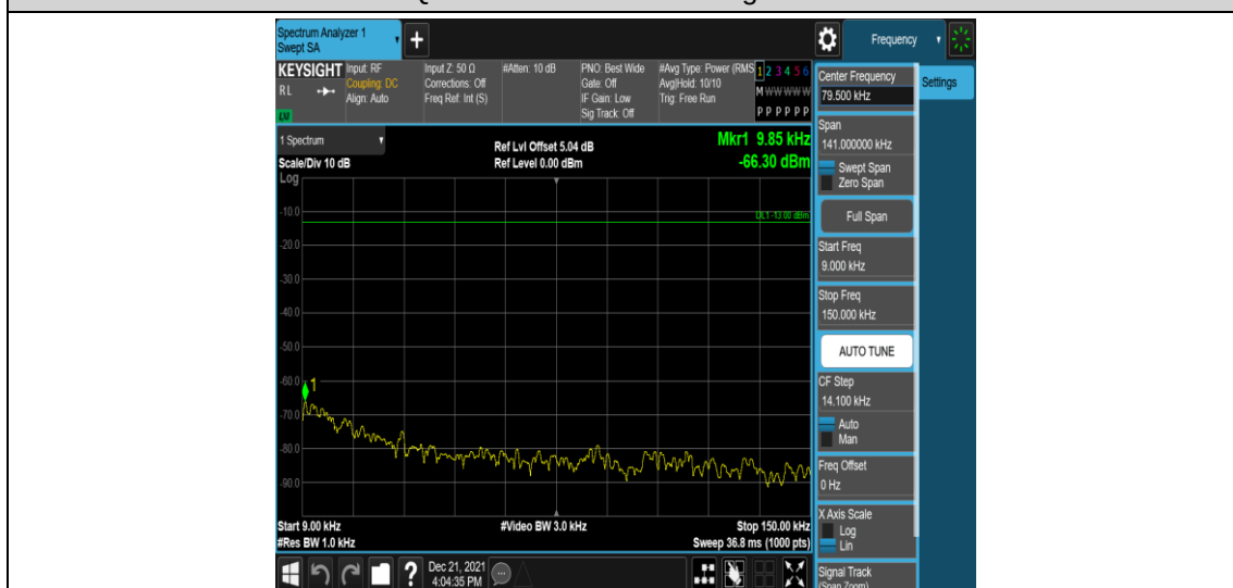
Band4-5MHz-16QAM-19975-1RB#0-Range1:0.009~0.15MHz
