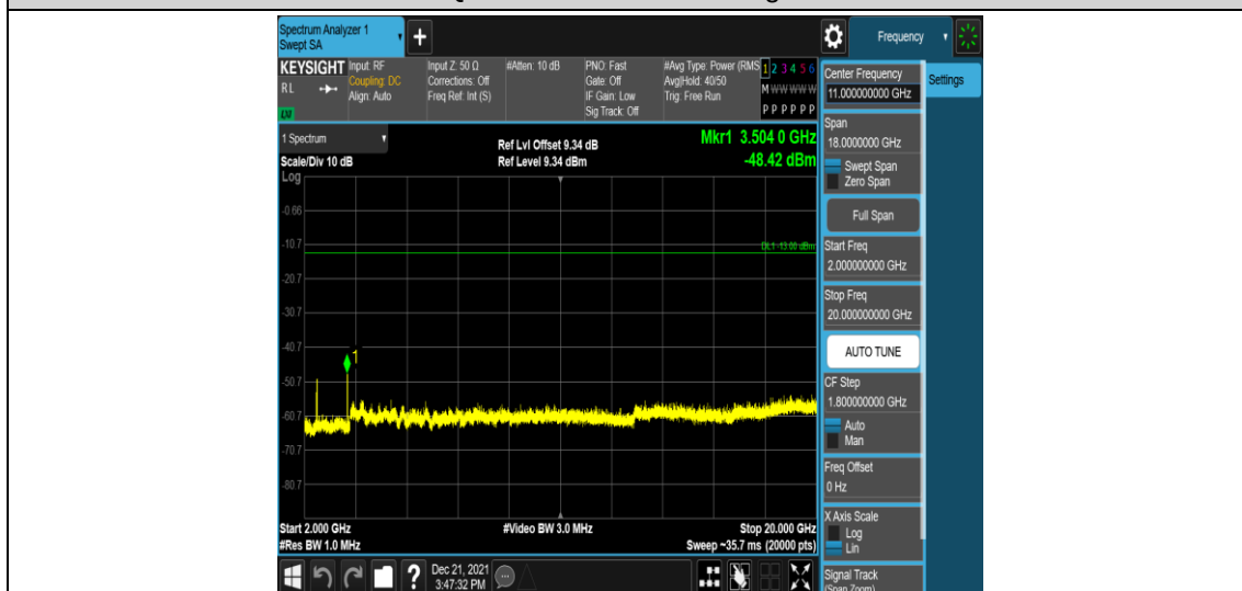
Band4-3MHz-16QAM-20385-1RB#0-Range5:2000~20000MHz
