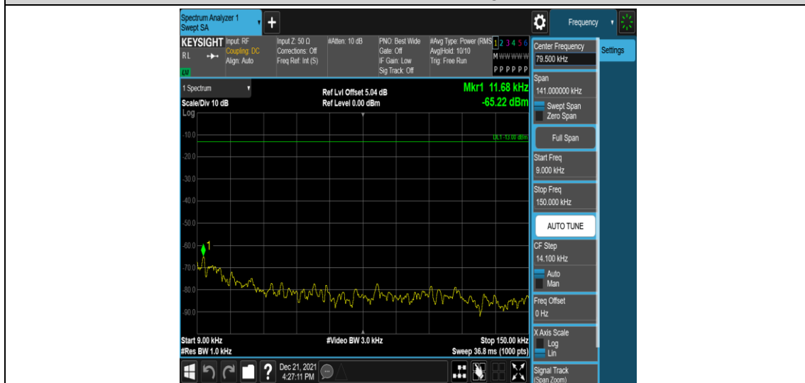
Band4-10MHz-QPSK-20175-1RB#0-Range1:0.009~0.15MHz
