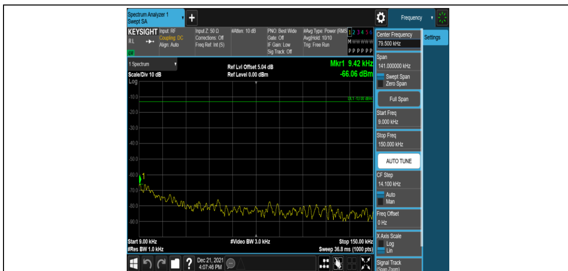
Band4-5MHz-QPSK-20375-1RB#0-Range1:0.009~0.15MHz
