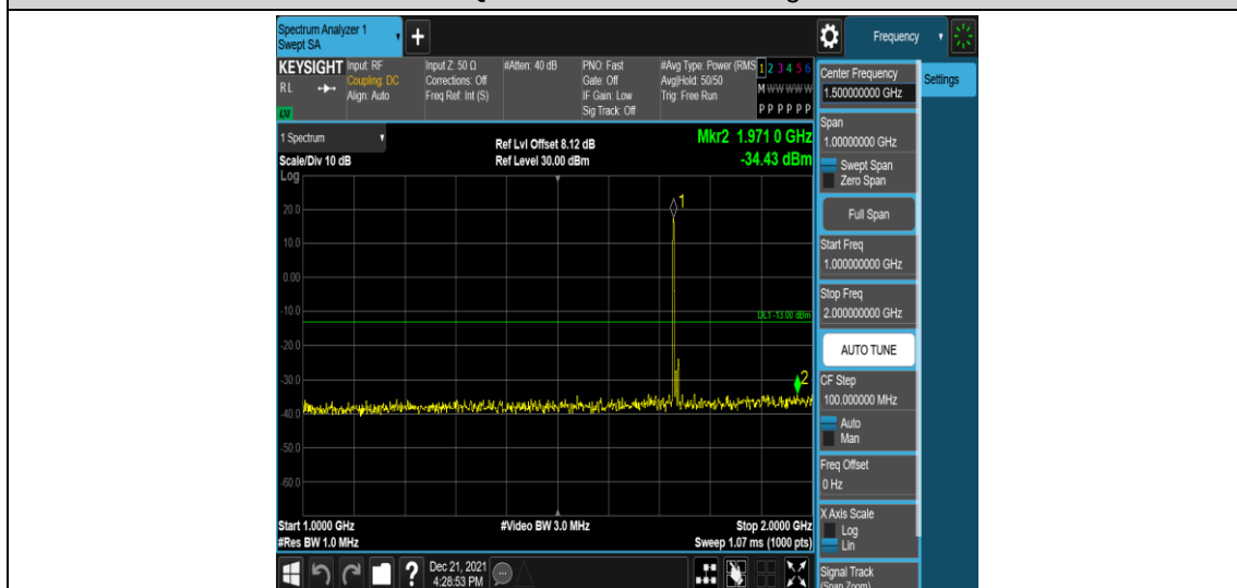
Band4-10MHz-16QAM-20175-1RB#0-Range4:1000~2000MHz
