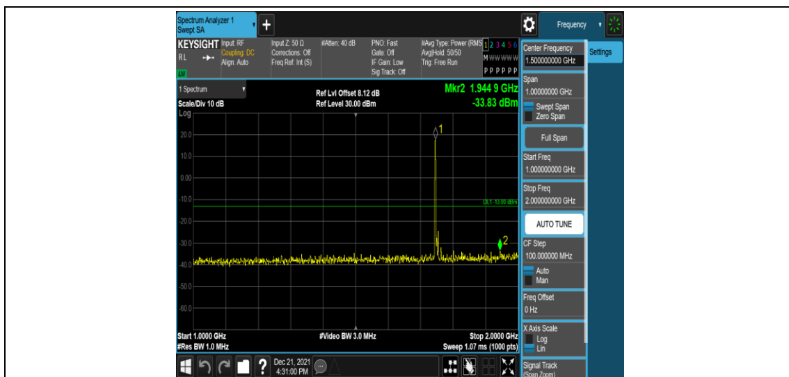
Band4-10MHz-16QAM-20350-1RB#0-Range4:1000~2000MHz
