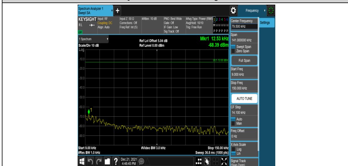
Band4-15MHz-QPSK-20025-1RB#0-Range1:0.009~0.15MHz
