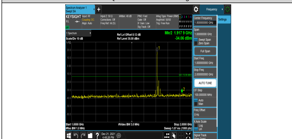
Band4-15MHz-16QAM-20025-1RB#0-Range4:1000~2000MHz
