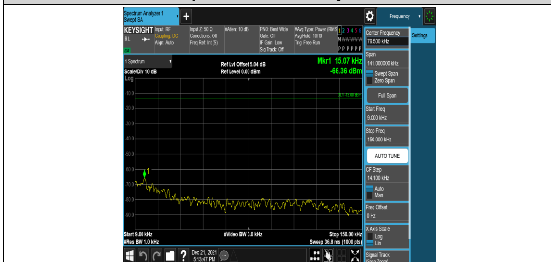
Band4-20MHz-QPSK-20175-1RB#0-Range1:0.009~0.15MHz
