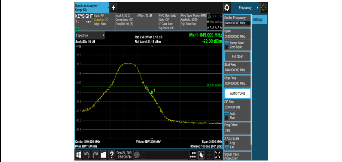
Band5-5MHz-QPSK-20625-1RB#24
