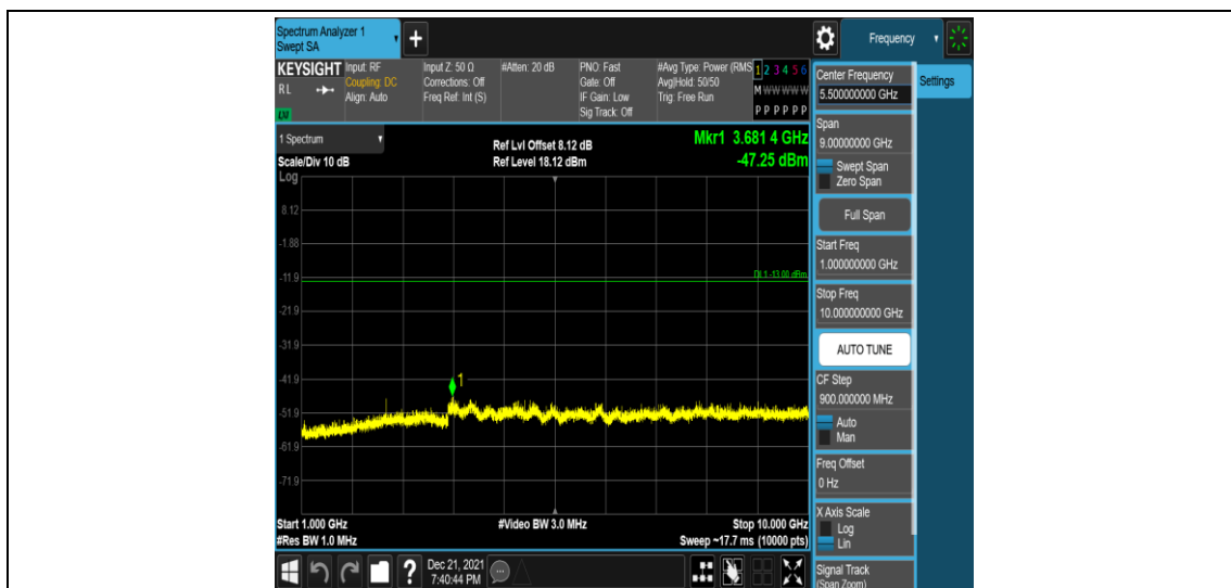
Band5-3MHz-QPSK-20525-1RB#0-Range4:1000~10000MHz
