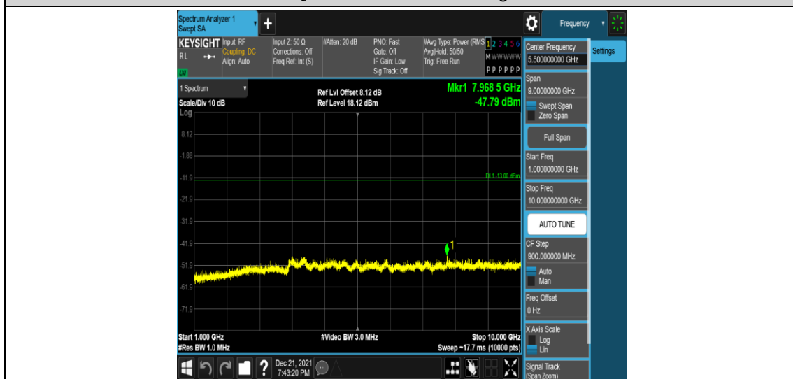
Band5-3MHz-16QAM-20635-1RB#0-Range4:1000~10000MHz
