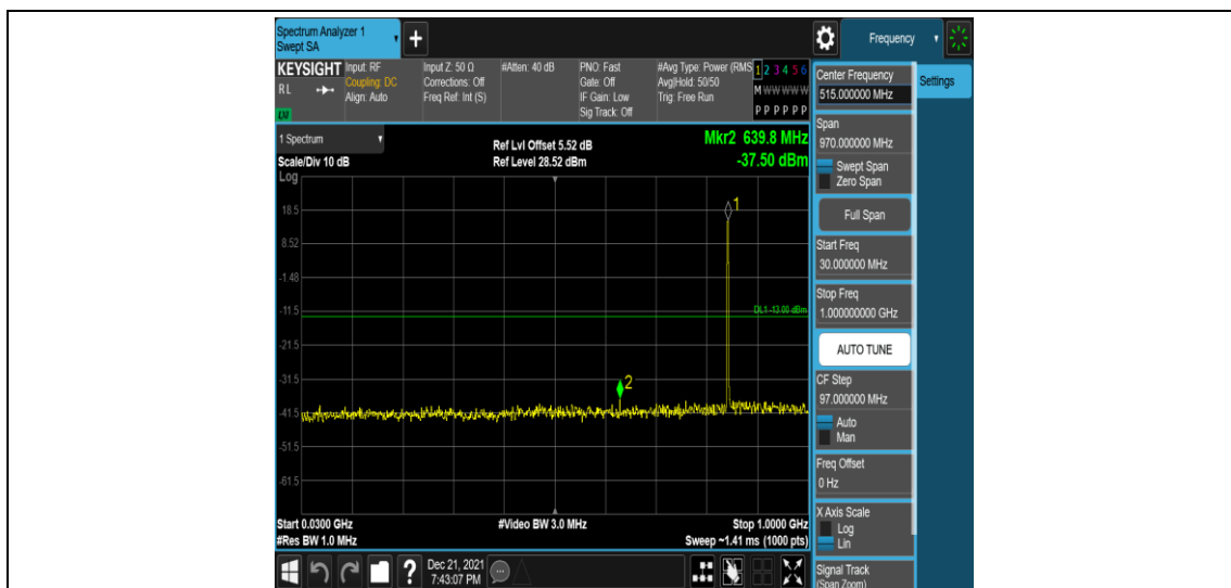
Band5-3MHz-16QAM-20635-1RB#0-Range3:30~1000MHz
