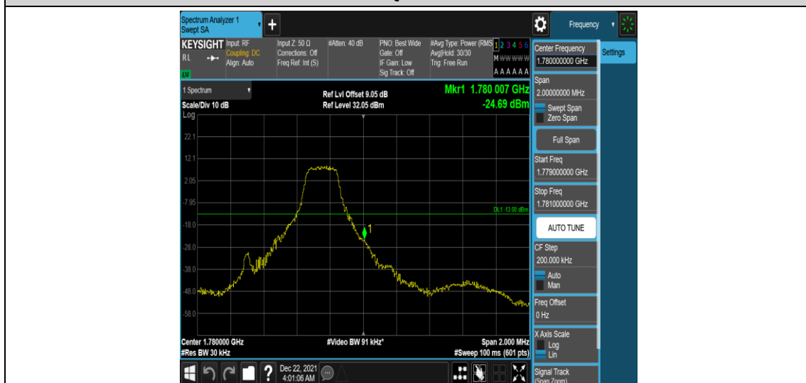
Band66-1.4MHz-QPSK-132665-1RB#5
