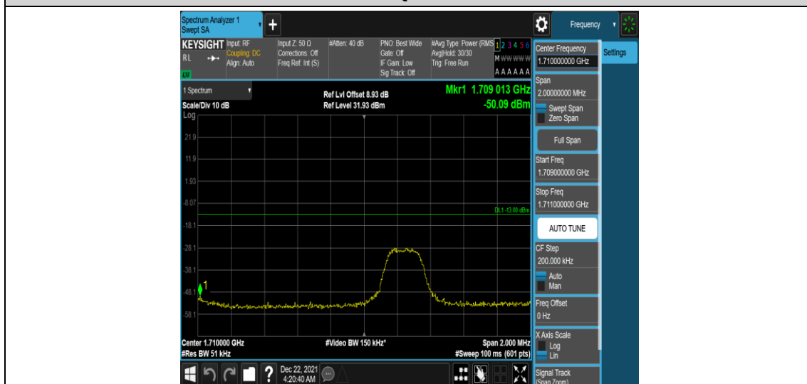
Band66-3MHz-16QAM-131987-1RB#14
