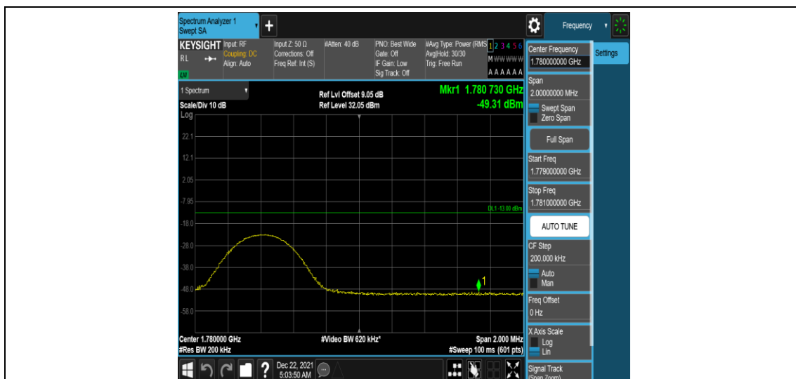
Band66-10MHz-QPSK-132622-1RB#0
