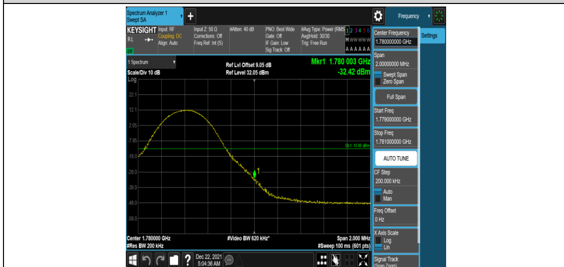
Band66-10MHz-16QAM-132622-1RB#49
