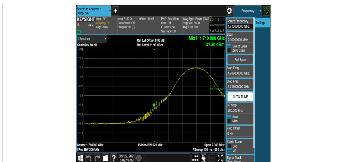
Band66-10MHz-16QAM-132022-1RB#0
