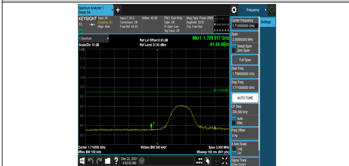
Band66-5MHz-16QAM-131997-1RB#24
