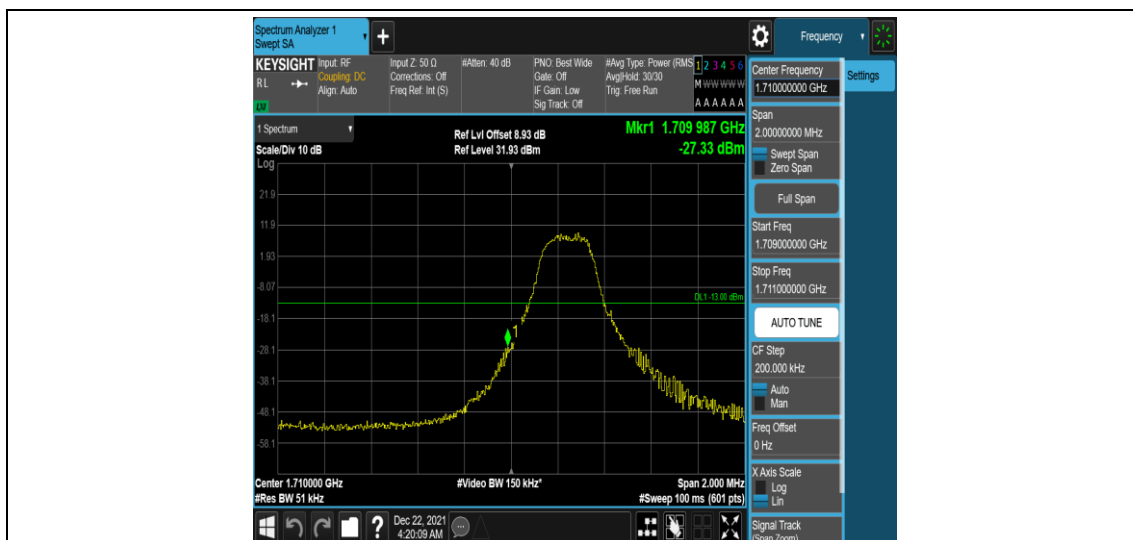
Band66-3MHz-16QAM-131987-1RB#0
