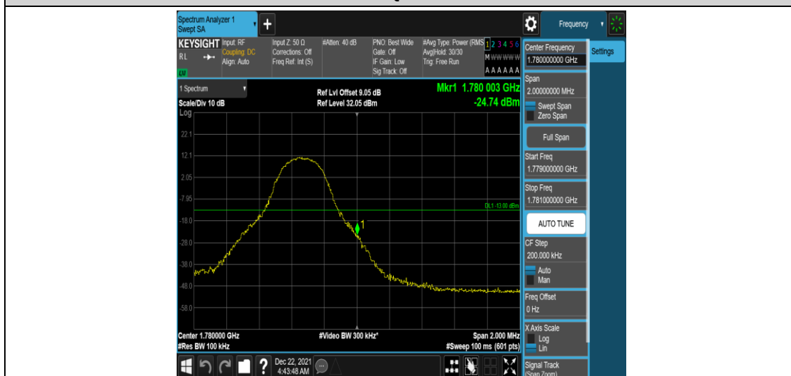
Band66-5MHz-16QAM-132647-1RB#24
