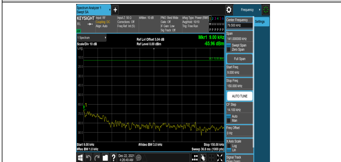
Band66-3MHz-QPSK-132657-1RB#0-Range1:0.009~0.15MHz
