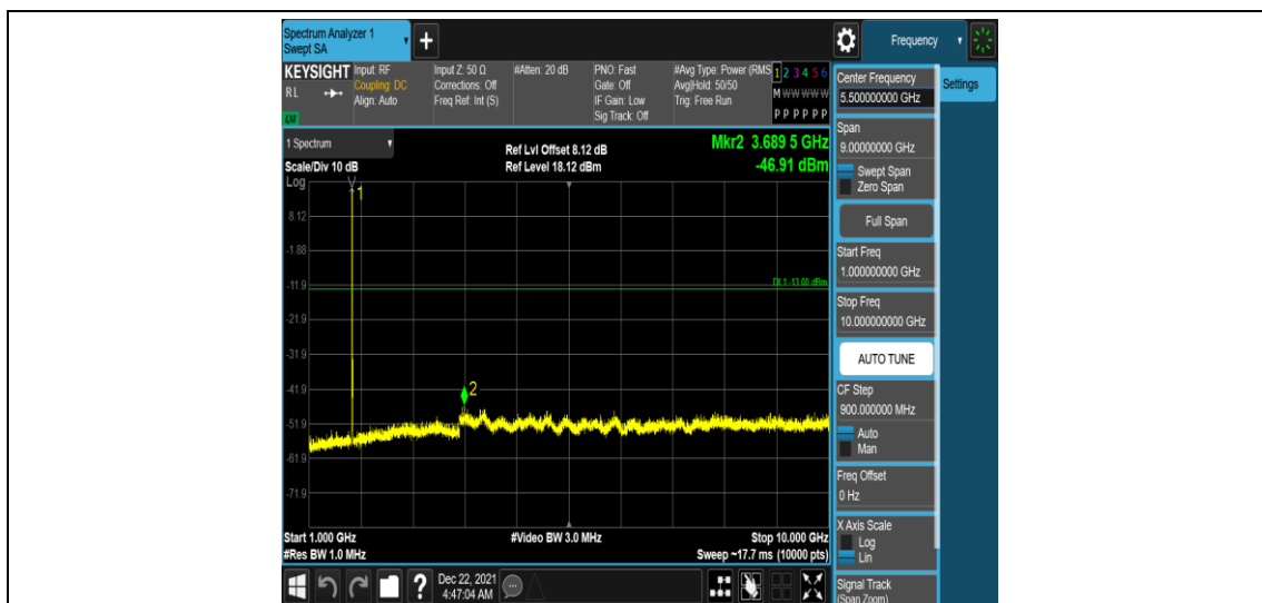
Band66-5MHz-QPSK-132322-1RB#0-Range4:1000~10000MHz
