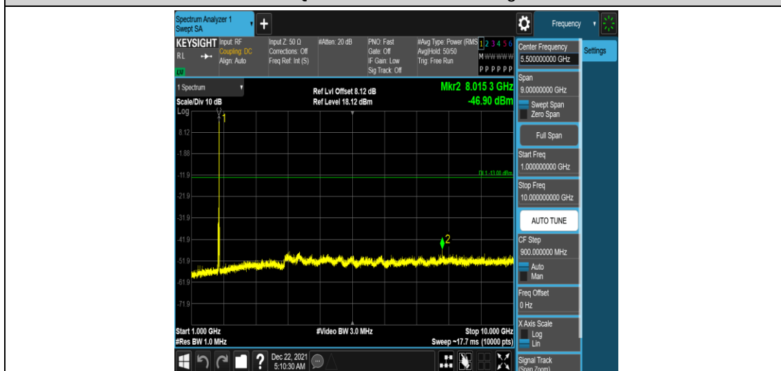
Band66-10MHz-16QAM-132622-1RB#0-Range4:1000~10000MHz
