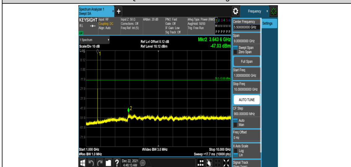
Band66-5MHz-16QAM-131997-1RB#0-Range4:1000~10000MHz
