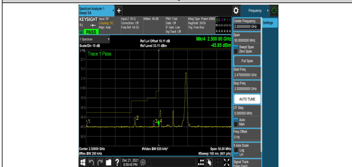
Band7-10MHz-16QAM-20800-1RB#49
