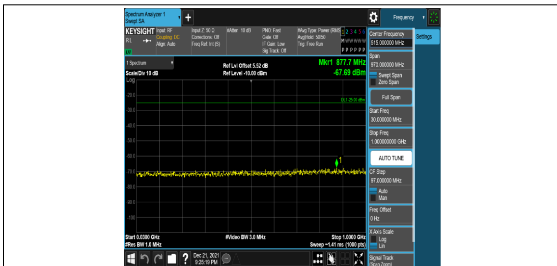
Band7-15MHz-QPSK-20825-1RB#0-Range3:30~1000MHz
