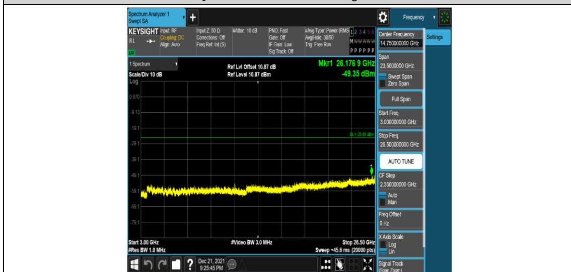
Band7-15MHz-QPSK-20825-1RB#0-Range5:3000~26500MHz
