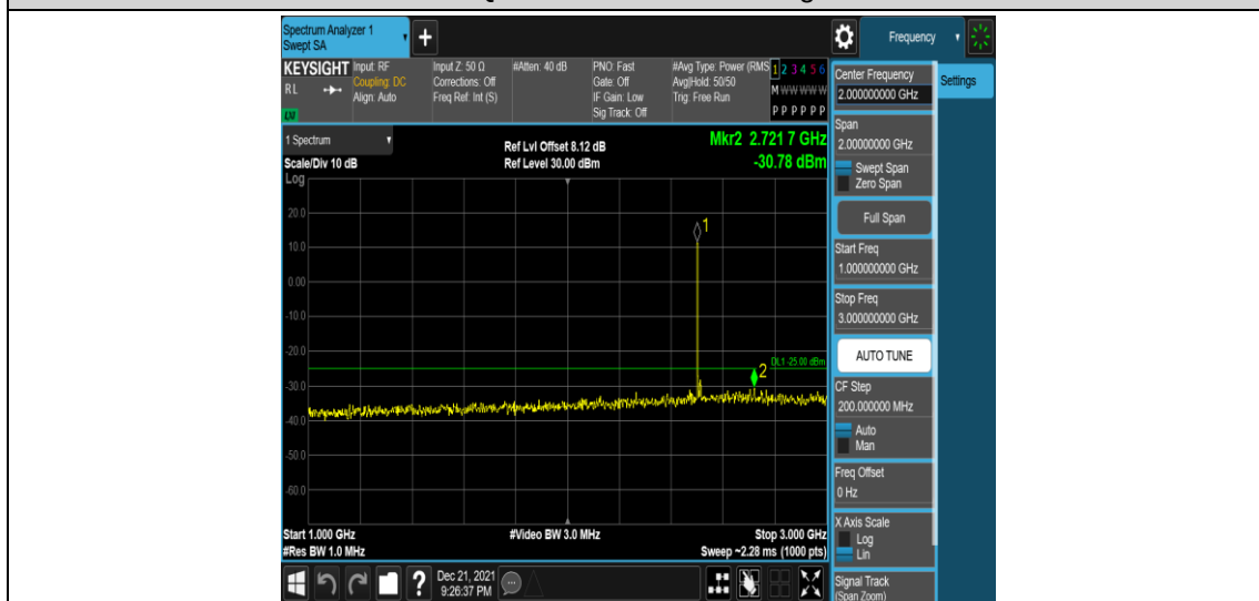
Band7-15MHz-16QAM-20825-1RB#0-Range4:1000~3000MHz
