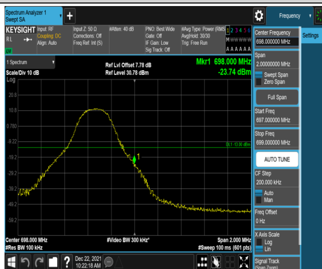
Band71-5MHz-16QAM-133447-1RB#24
