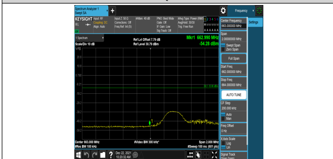
Band71-5MHz-16QAM-133147-1RB#24
