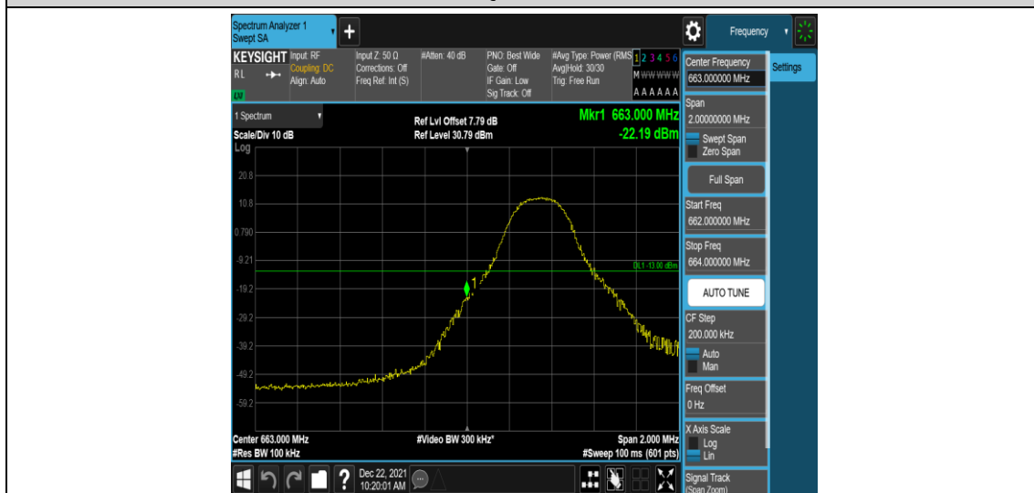
Band71-5MHz-16QAM-133147-1RB#0
