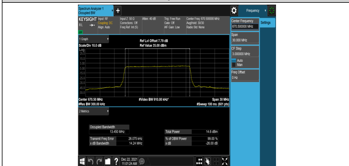
Band71-15MHz-16QAM-133197-75RB#0
