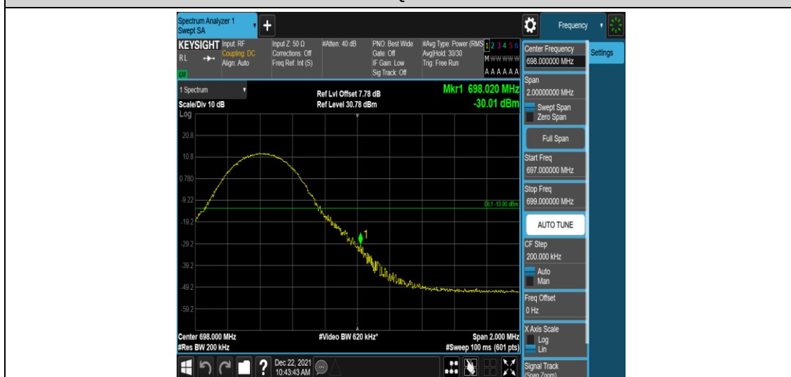
Band71-10MHz-16QAM-133422-1RB#49
