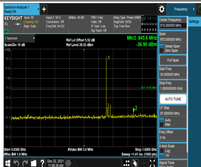
Band71-15MHz-QPSK-133197-1RB#0-Range3:30~1000MHz
