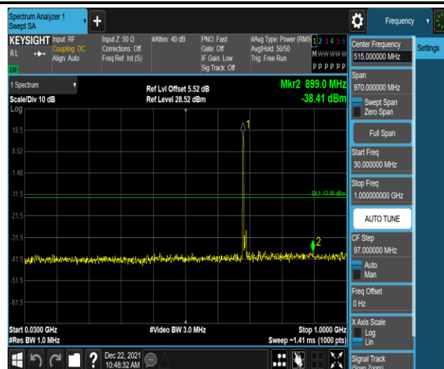
Band71-10MHz-QPSK-133422-1RB#0-Range3:30~1000MHz
