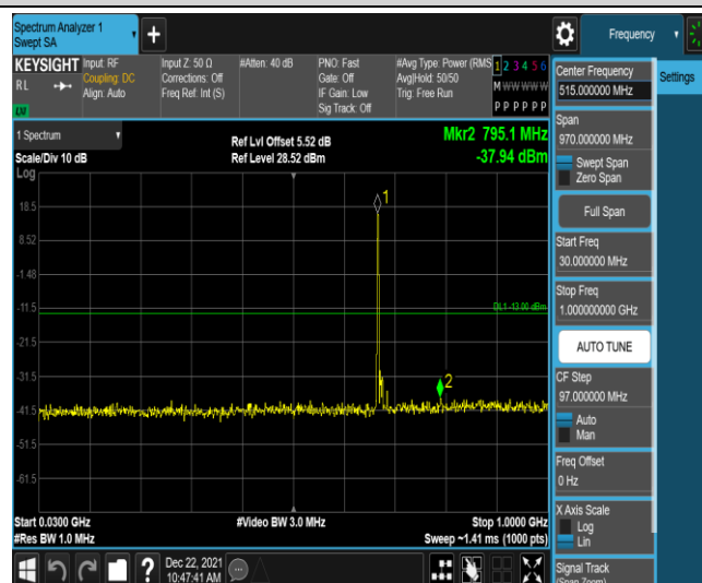
Band71-10MHz-16QAM-133297-1RB#0-Range3:30~1000MHz
