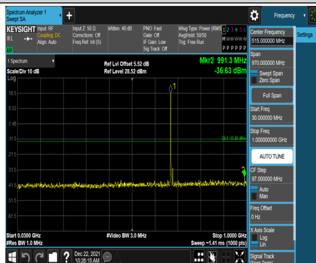
Band71-5MHz-16QAM-133297-1RB#0-Range3:30~1000MHz
