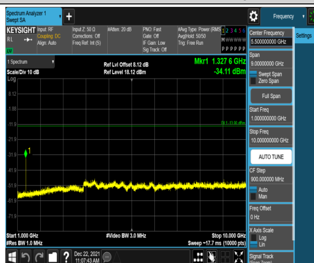
Band71-15MHz-16QAM-133197-1RB#0-Range4:1000~10000MHz
