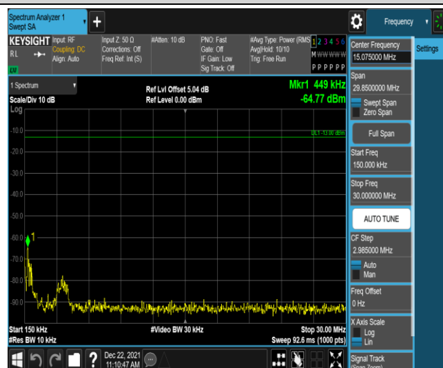
Band71-15MHz-16QAM-133397-1RB#0-Range2:0.15~30MHz
