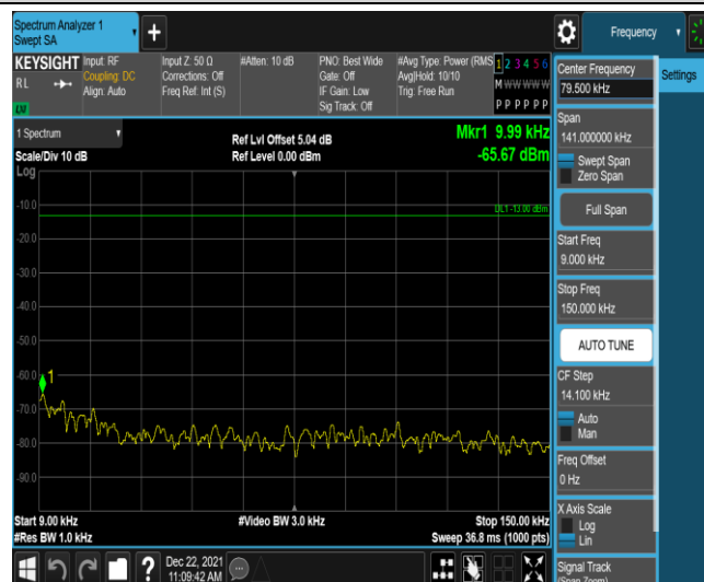
Band71-15MHz-QPSK-133397-1RB#0-Range1:0.009~0.15MHz
