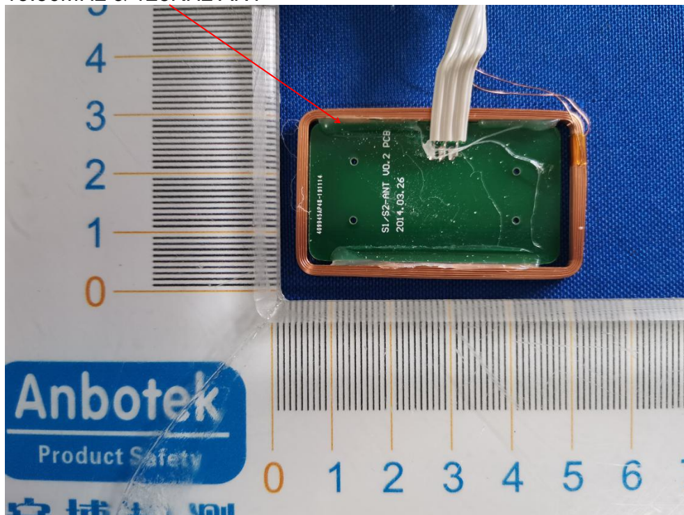
13.56MHz & 125KHz ANT
