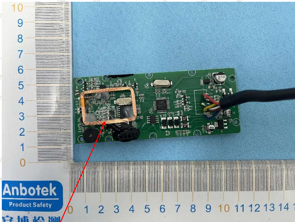
125kHz ANT
