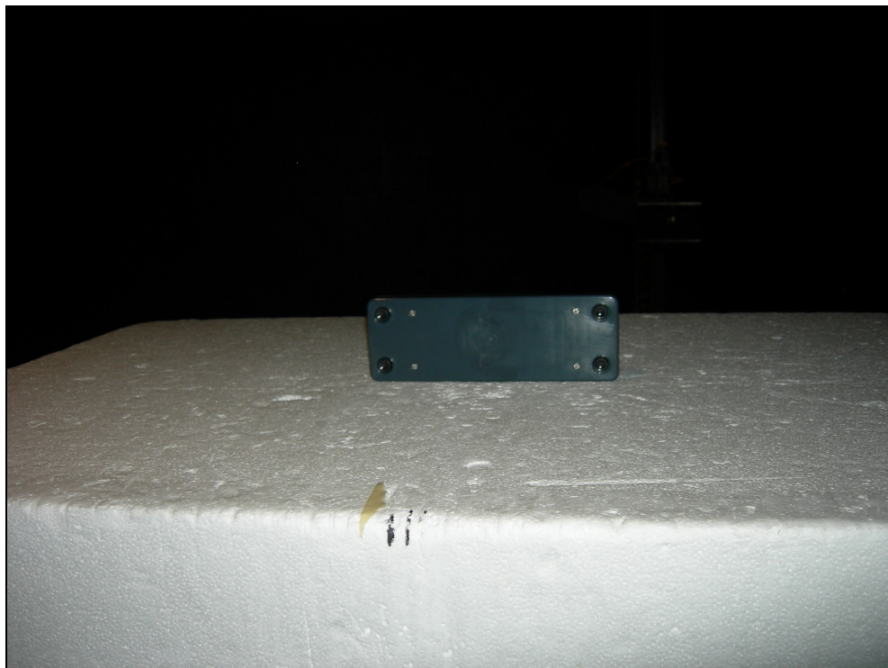
Figure 7: Radiated Emissions – ZPOS
